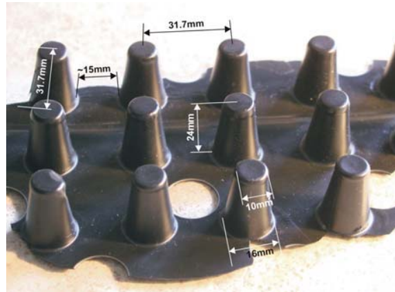
Figure 3.5: Akwadrain plastic substrate
