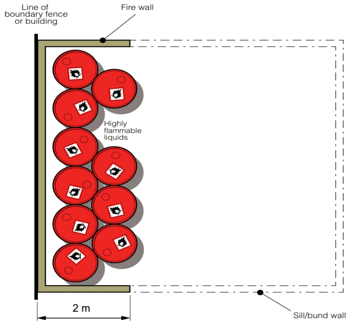
Figure 2.1.5.1.b - Separation distance for highly flammable liquids in drums and similar portable containers stored outside (viewed from above).
