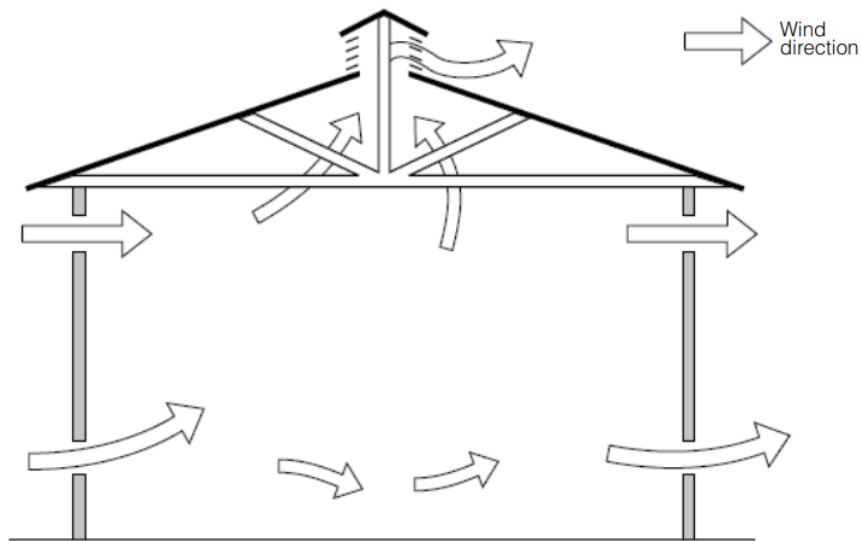
Figure 2.1.5.5 – Roof and Wall Ventilation.
