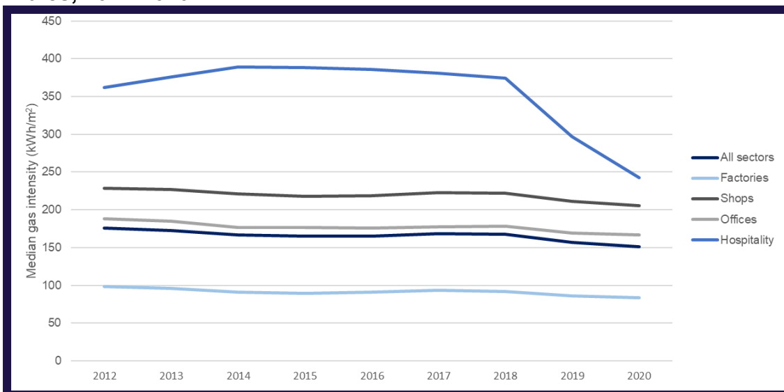
Figure 34: Median gas intensity in ND-NEED non-domestic buildings in England and Wales, 2012-2020.
