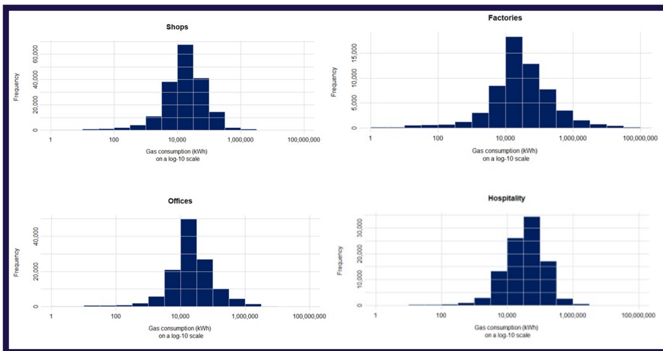
Figure 16: Frequency of different gas consumption values, split by building use, 2020.
