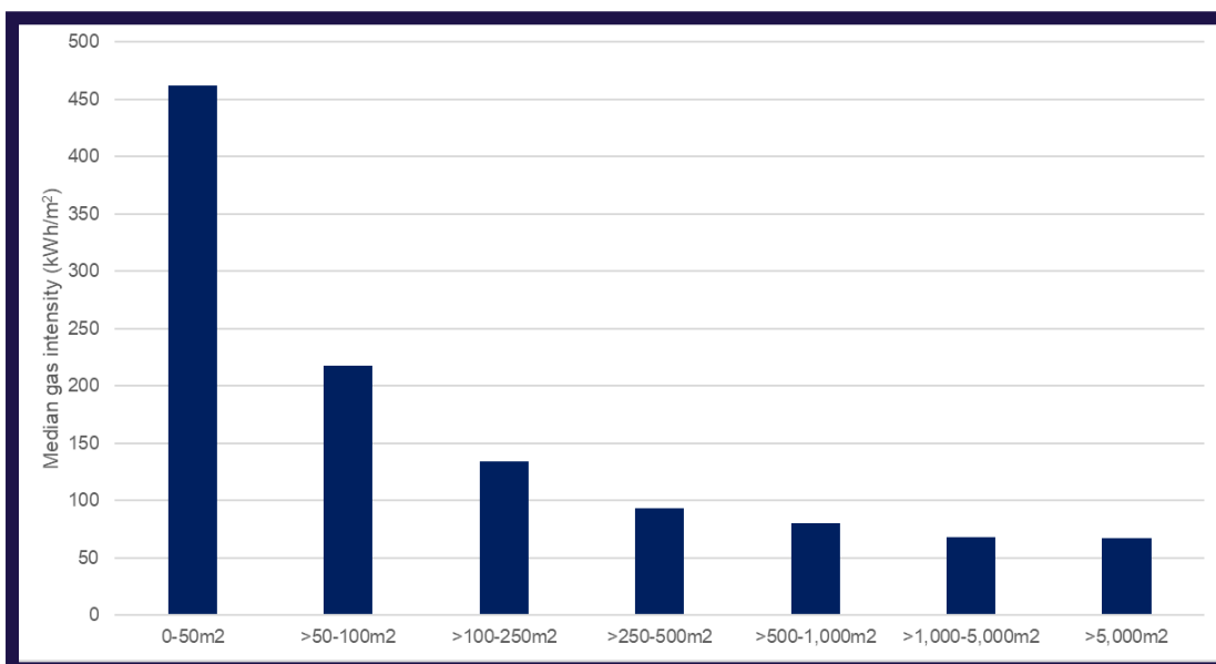
Figure 24: The median gas intensity of ND-NEED non-domestic buildings in England and Wales by building size, 2020.
