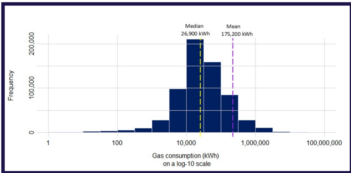
Figure 15: Frequency of different gas consumption values for all non-domestic buildings, 2020.
