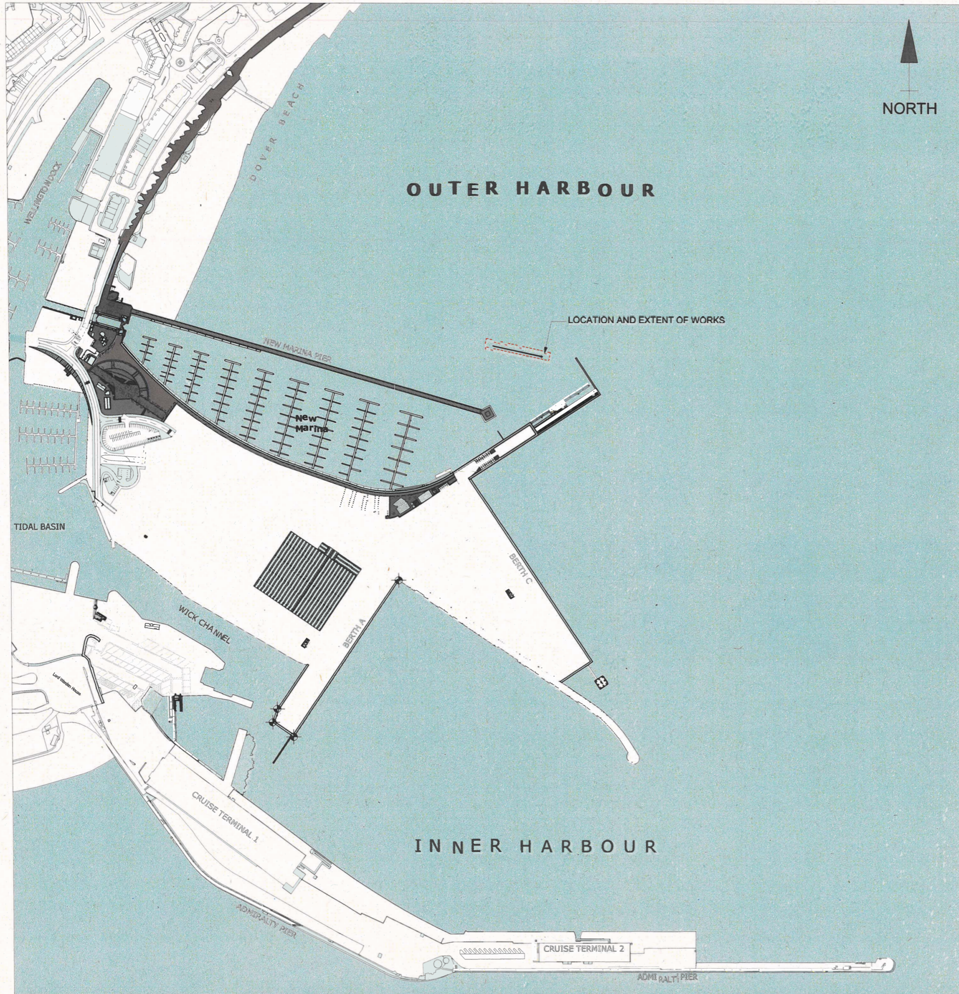
LOCATION AND EXTENT OF WORKS Scale 1:2500 @ A1
