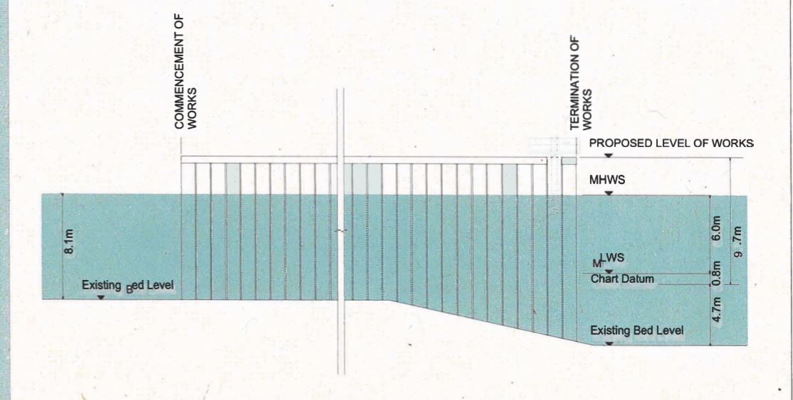
SECTION ALONG CENTRELINE OF WORKS Scale 1:200 @ A1
