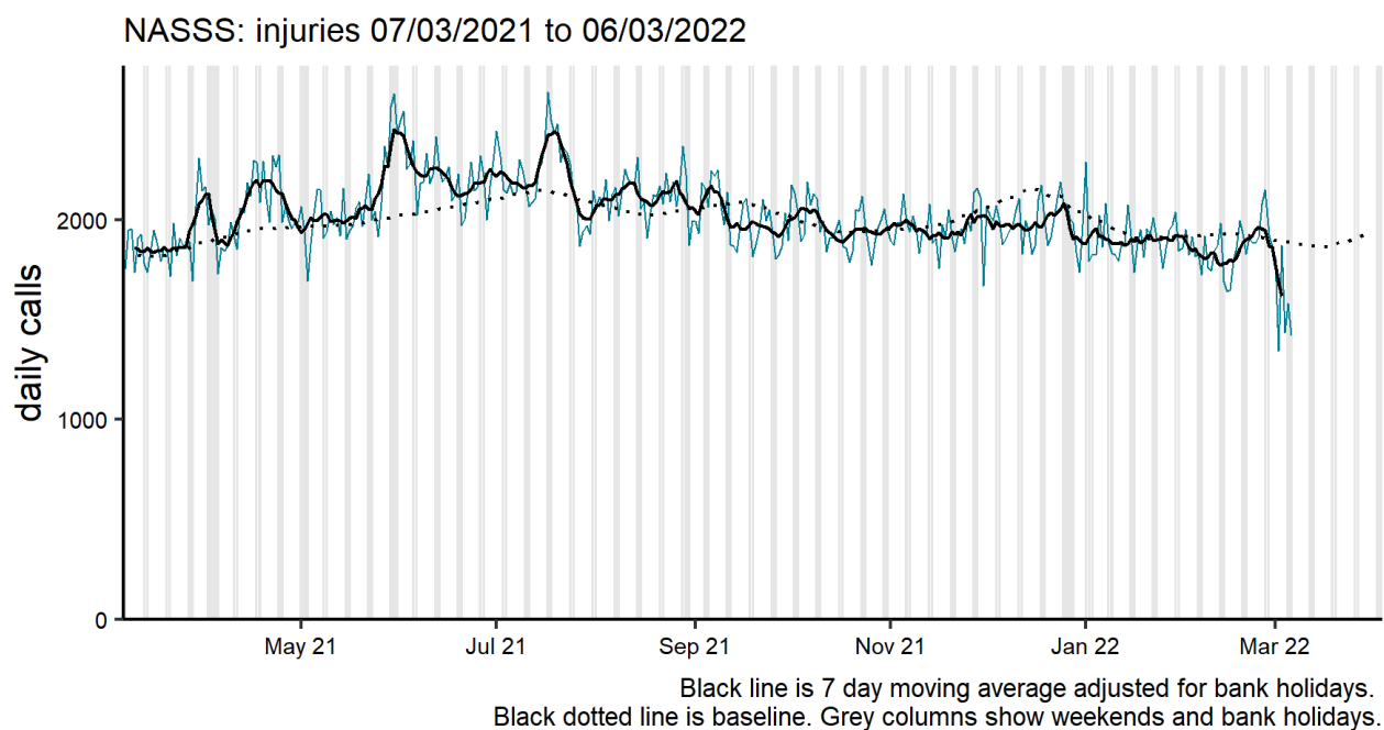
Figure 10: Daily number of injury ambulance service calls (and 7-day moving average adjusted for bank holidays), England (a) nationally, (b) by UKHSA Region.
