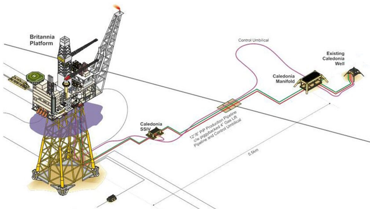
Figure 1.1: Caledonia Field Schematic
