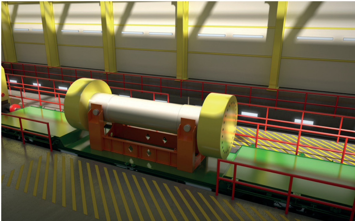
Figure 2: A package of spent fuel on a rail wagon. The waste package destined for a GDF is contained within an outer transport container, with 'impact limiters' on each end to provide added protection during its journey to the GDF.
