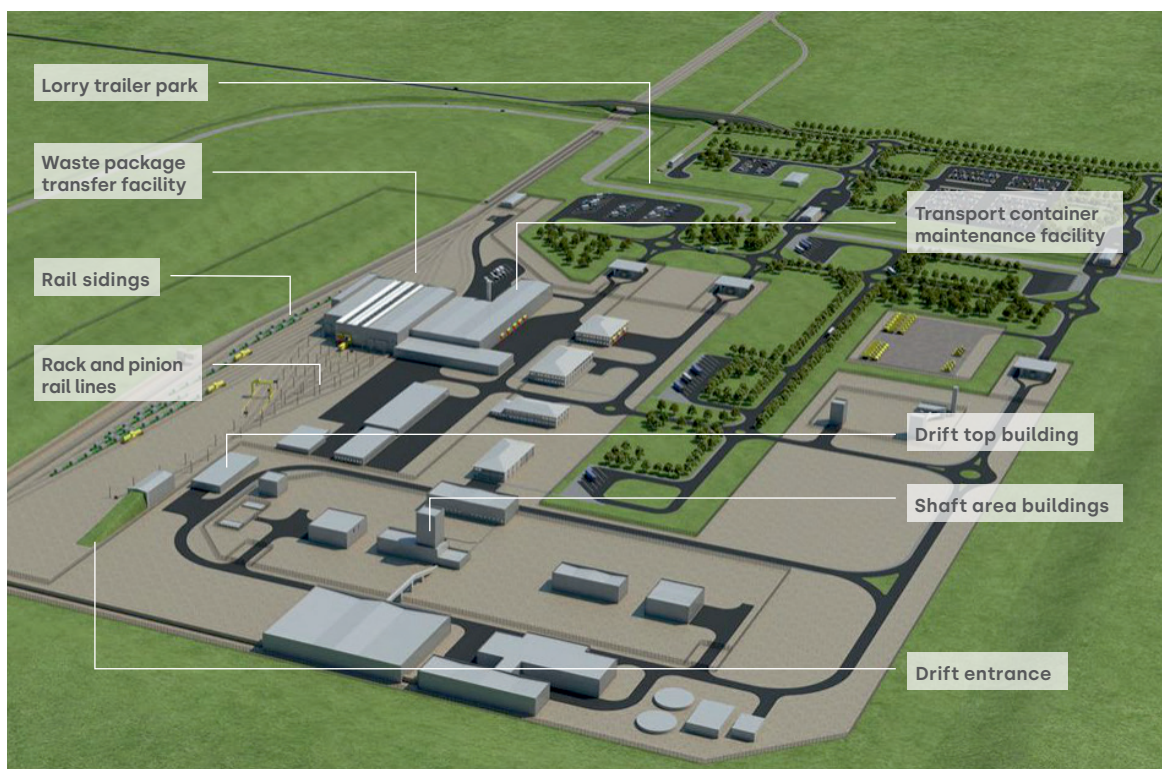
Figure 1: An illustrative aerial view of a GDF surface layout.
