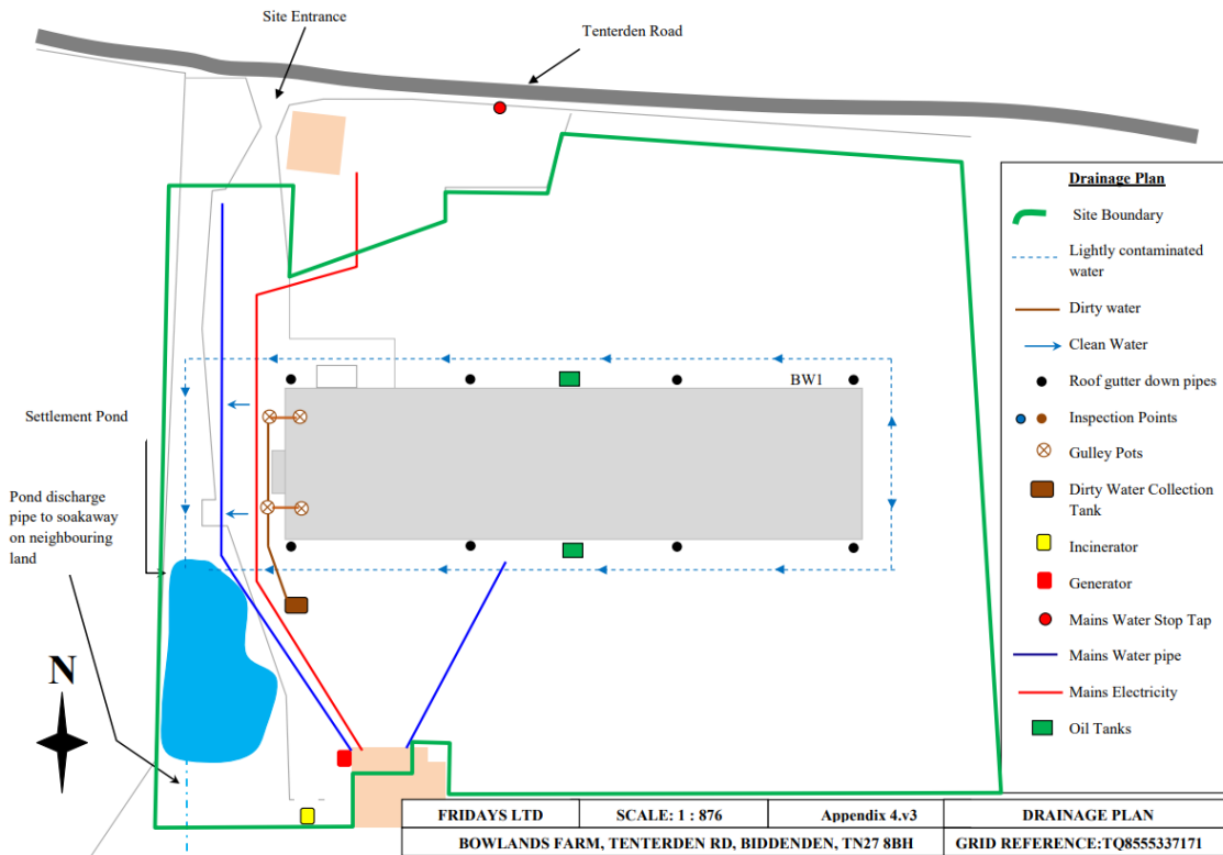
Site drainage plan
