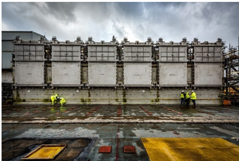
Figure 42: Penetrations into each PFCS compartment, each sealed with a steel door
