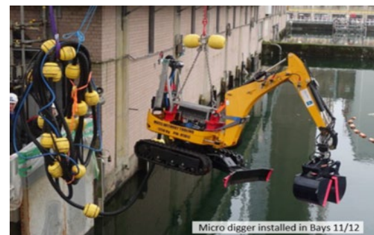
Figure 36: A micro-digger used to clear solid debris from PFSP bays 11 and 12.
