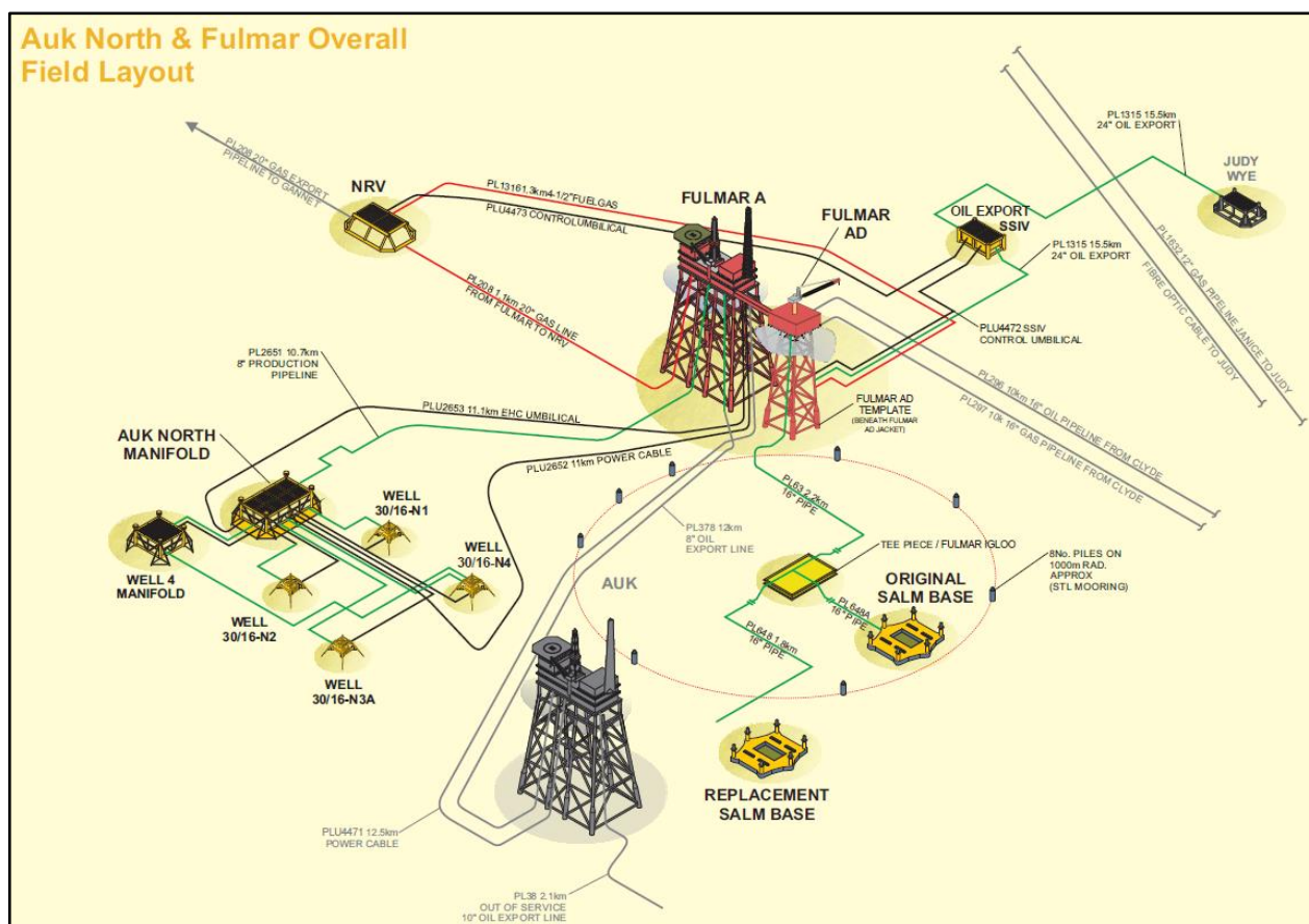
Figure 1.2: Field Layout Note 1 & 2
