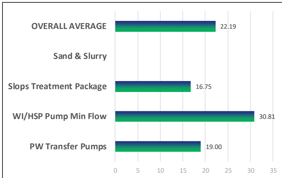
Figure 4: Average oil concentration in produced water by discharge route (mg/l) in 2020.
