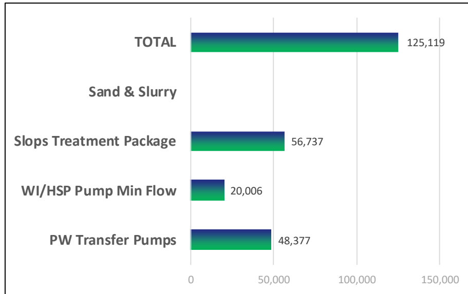
Figure 5: Volume of produced water discharged to sea via each discharge route (m 3 ) in 2020.
