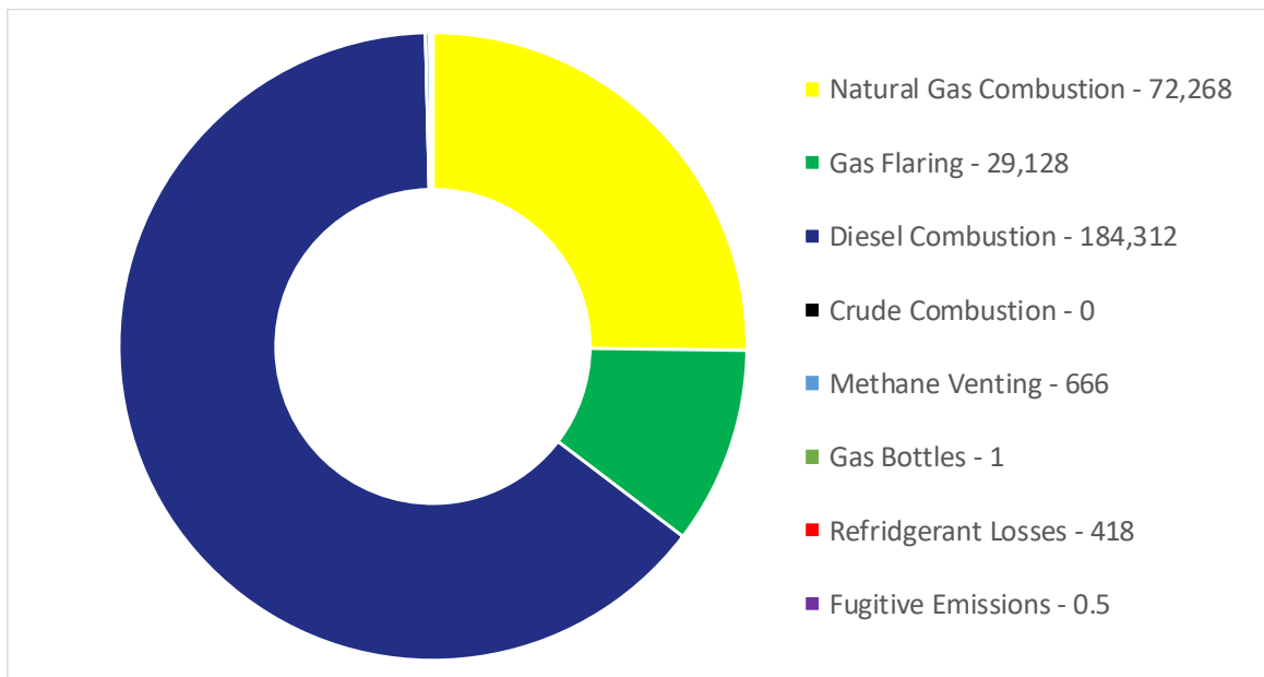
Figure 10: Armada Kraken GHG emissions CO 2 equivalent (tonnes).
