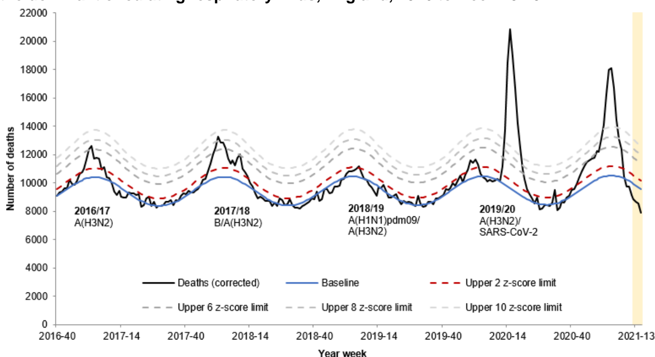
Figure 1: Weekly observed and expected number of all-cause deaths in all ages, with the dominant circulating respiratory virus, England, 2016 to week 15 2021
