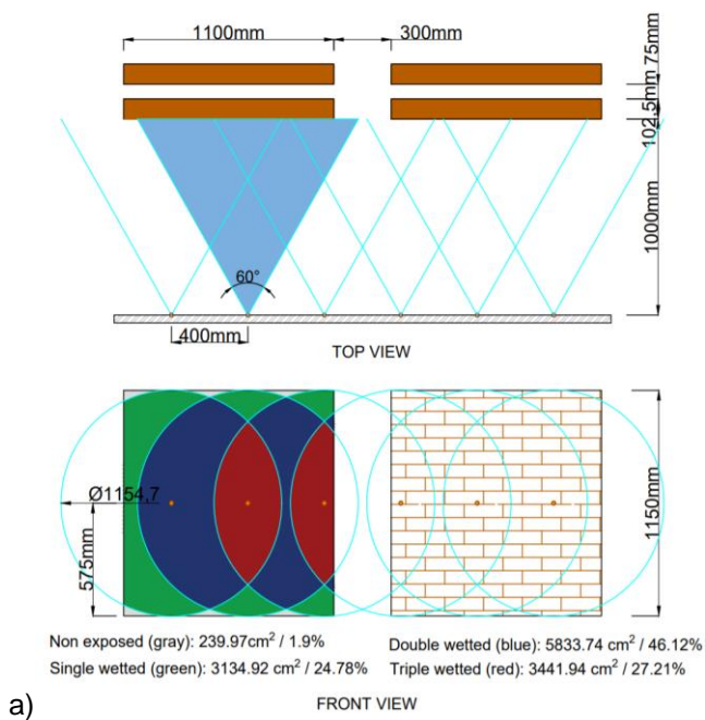
Figure 8: a) Theoretical patterns of wetting of walls during WDR tests b) Calibration of water distribution with WDR gauges
