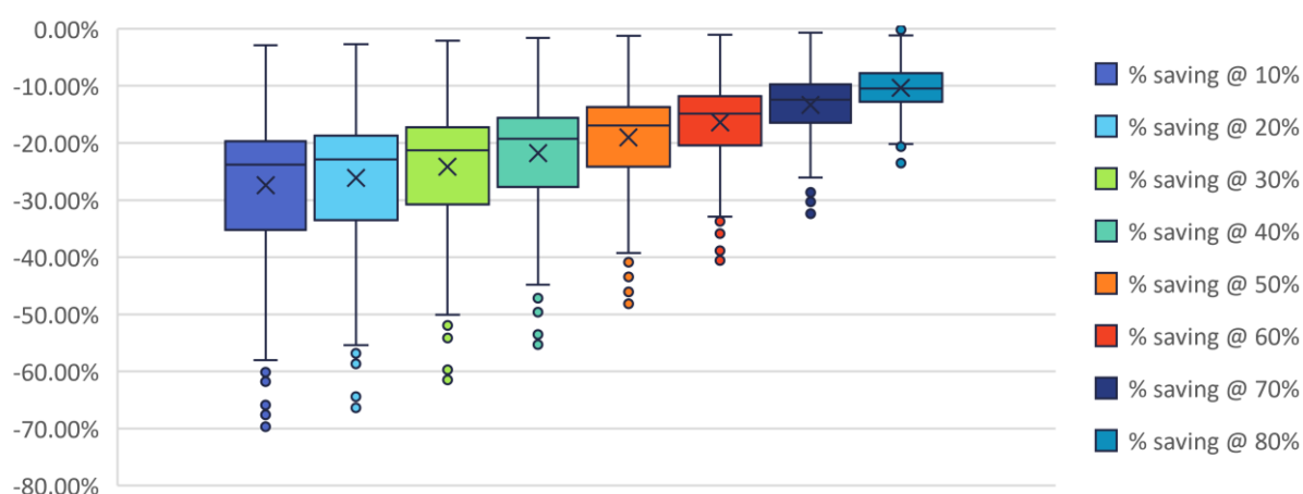
Figure 5-1 Solid wall, all archetypes: modelled reduction in heating energy from IWI, percentage glazing as variable parameter
