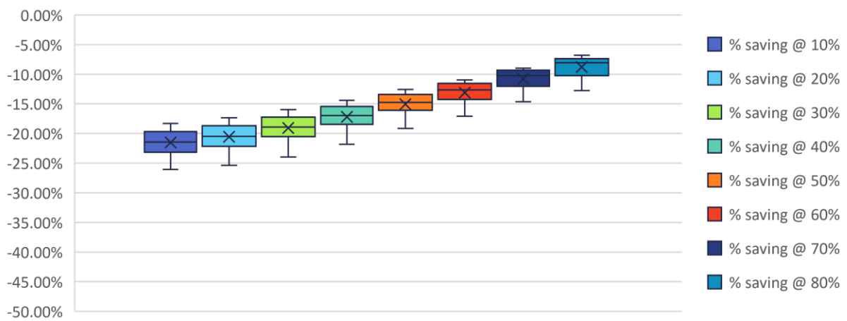
Solid wall, all archetypes, TIWI 5: predicted savings in heating energy consumption, percentage glazing as variable parameter
