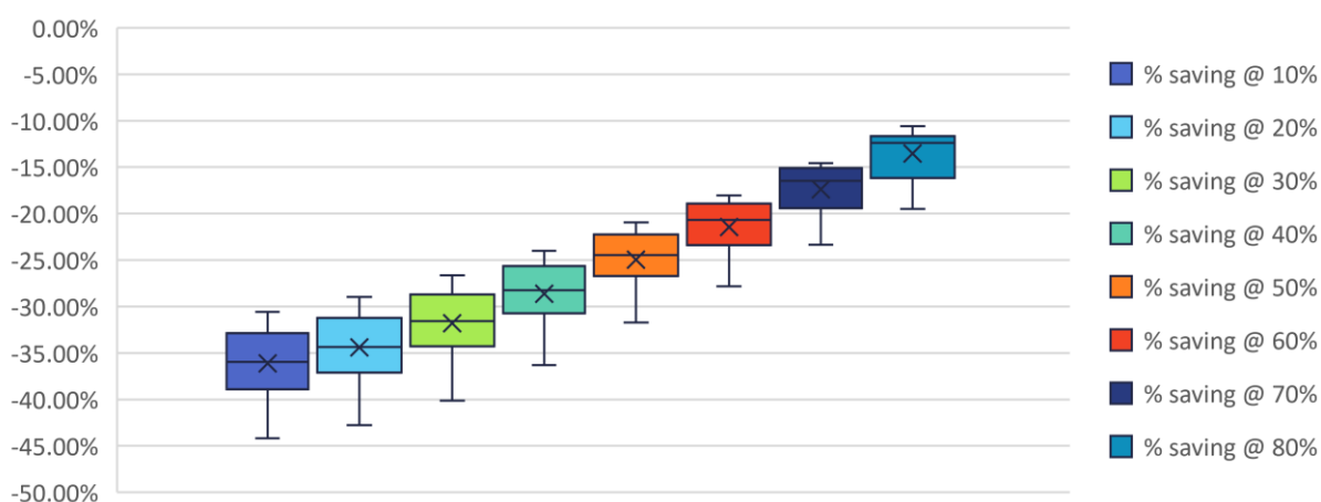
Solid wall, all archetypes, TIWI 2: modelled reduction in heating energy, percentage glazing as variable parameter
