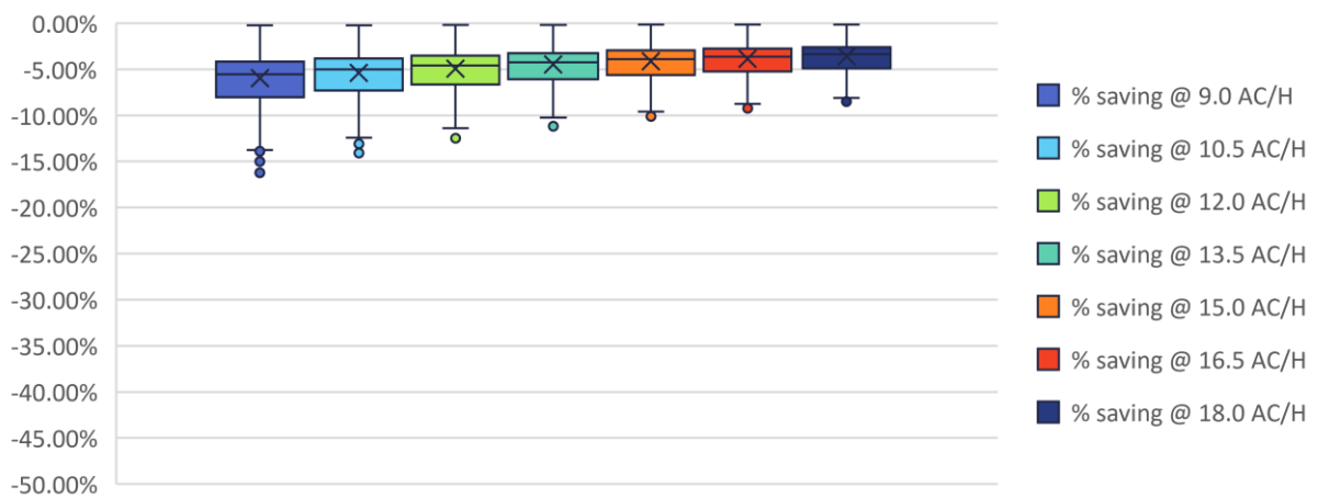
Insulated cavity wall, all archetypes, TIWI average: modelled reduction in heating energy, air changes as variable parameter
