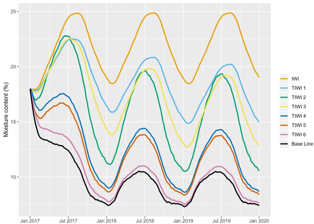
Figure 3-4 Water content in masonry inner leaf
