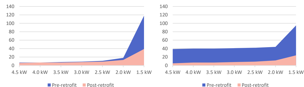
(a) Minutes below 21°C – air temperature (b) Minutes below 18°C – operative temperature Figure 4-24 Summary of radiator sizing sensitivity analysis results for Test House B
