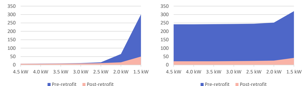
(a) Minutes below 21°C – air temperature (b) Minutes below 18°C – operative temperature Figure 4-25 Summary of radiator sizing sensitivity analysis results for Test House C
