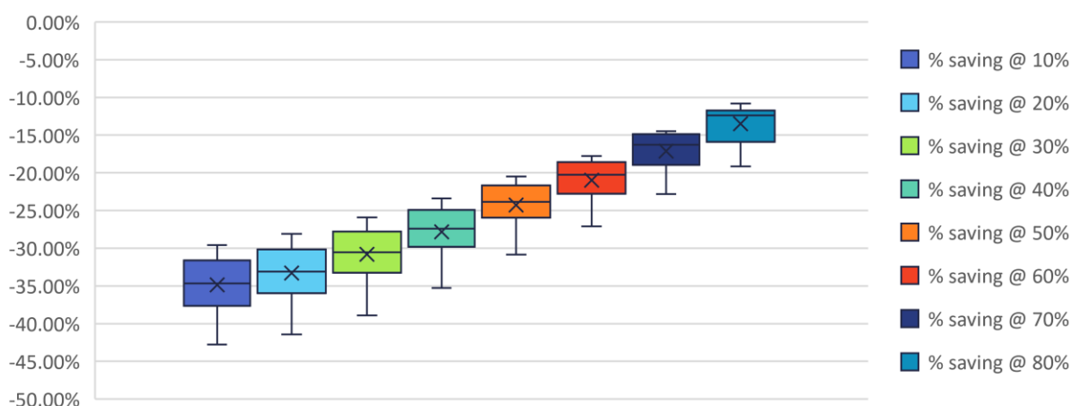
Solid wall, all archetypes, TIWI 1: modelled reduction in heating energy, percentage glazing as variable parameter
