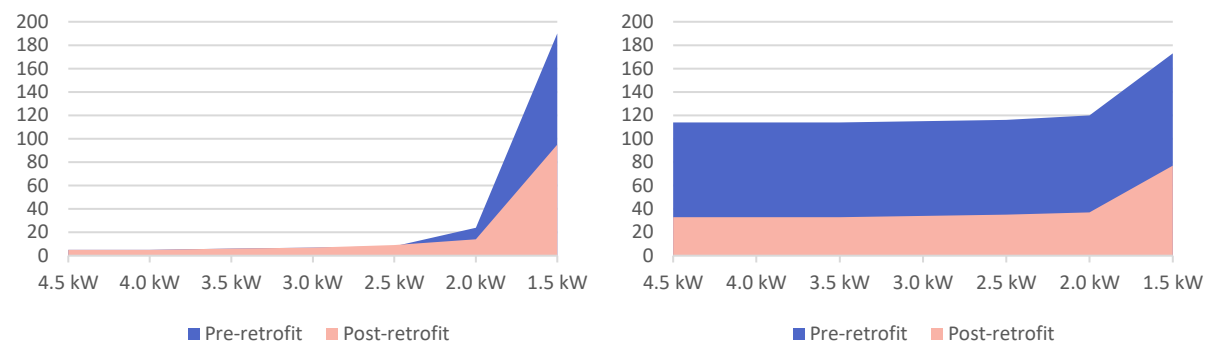
(a) Minutes below 21°C – air temperature (b) Minutes below 18°C – operative temperature Figure 4-23 Summary of radiator sizing sensitivity analysis results for Test House A
