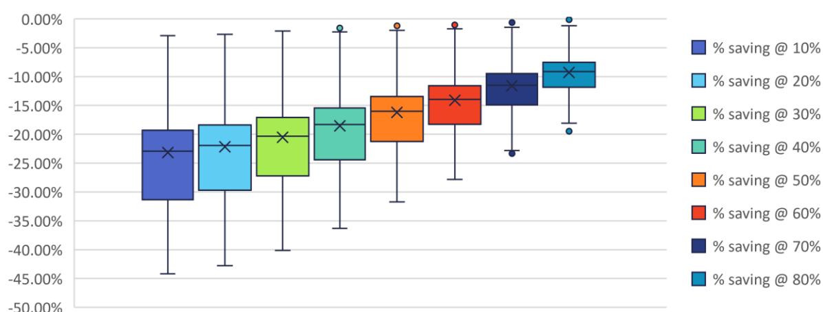
Figure 5-2 Solid wall, all archetypes, modelled reduction in heating energy from TIWI, percentage glazing as variable parameter
