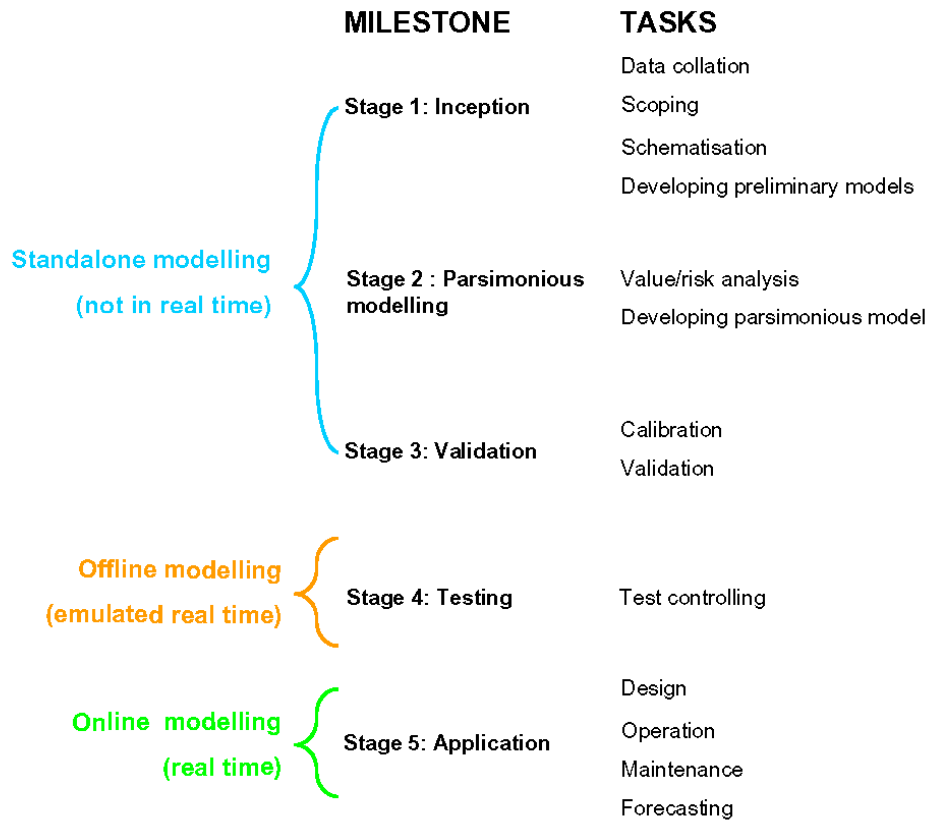
Figure 2. Stages in the model building and testing cycle for flood forecasting models proposed by the National Flood Forecasting Systems Strategy.
