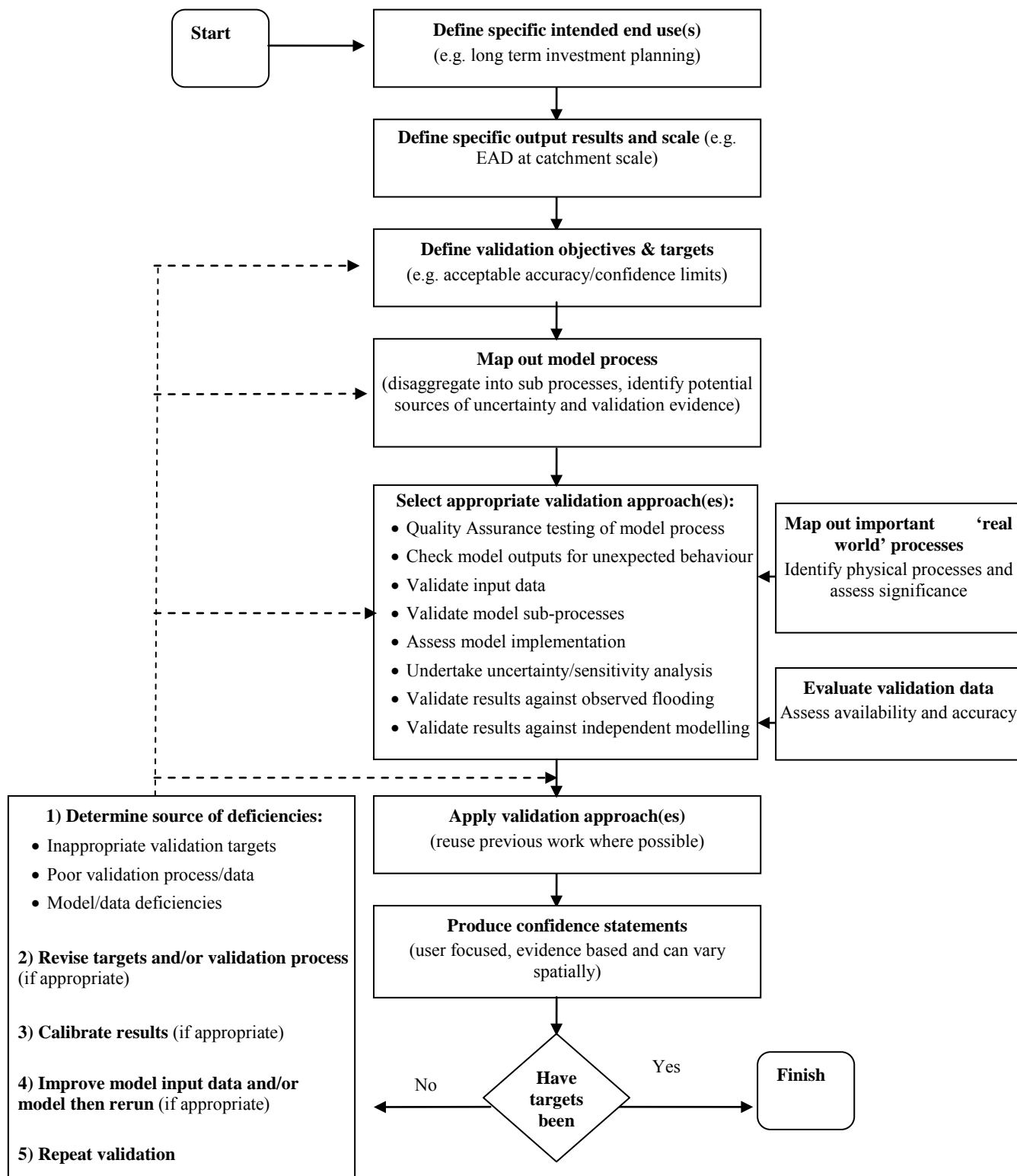
Figure 1: High level validation framework for probabilistic flood models.
