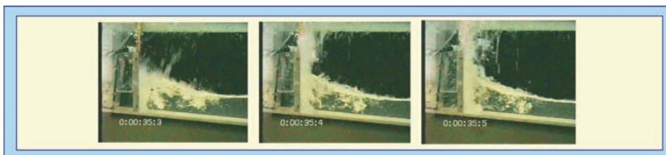
Fig. 7.5: A broken wave at a vertical wall, resulting in a broken wave overtopping condition
