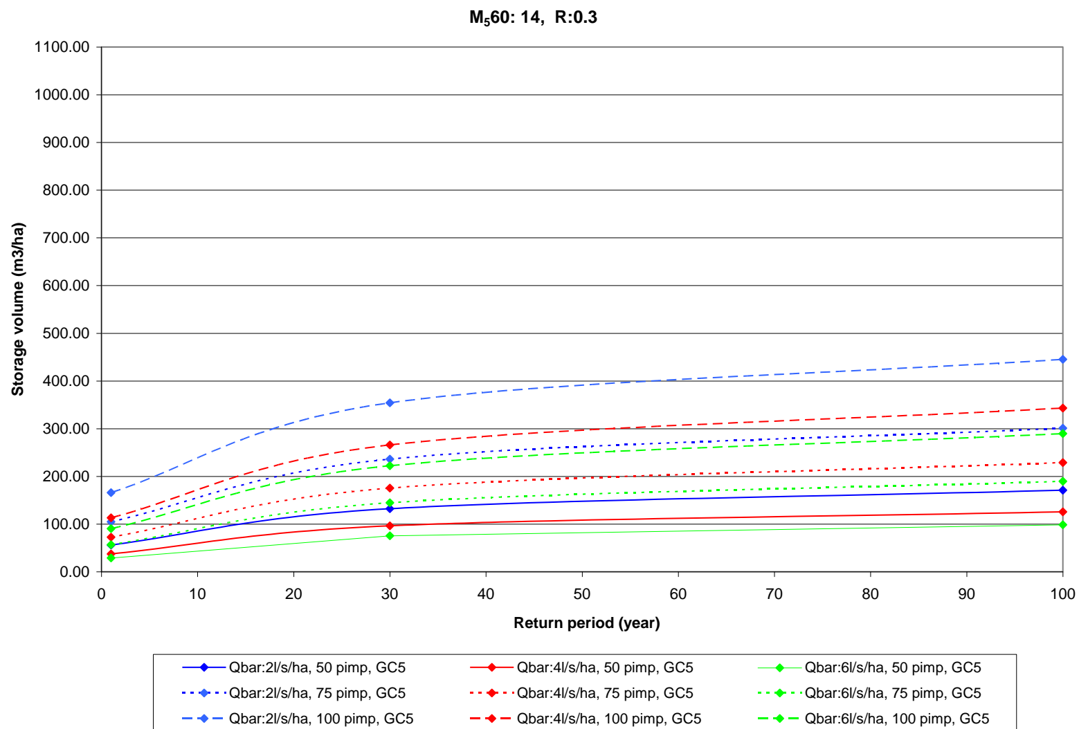
Figure A7.2 Attenuation storage volume as a function of Q_{\text{BAR}}/A and PIMP (M 5 60:14, “r”:0.3)
