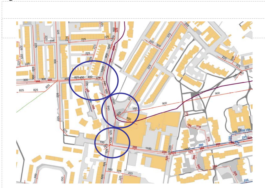
Figure 4 Hot-spots in a sewer system
