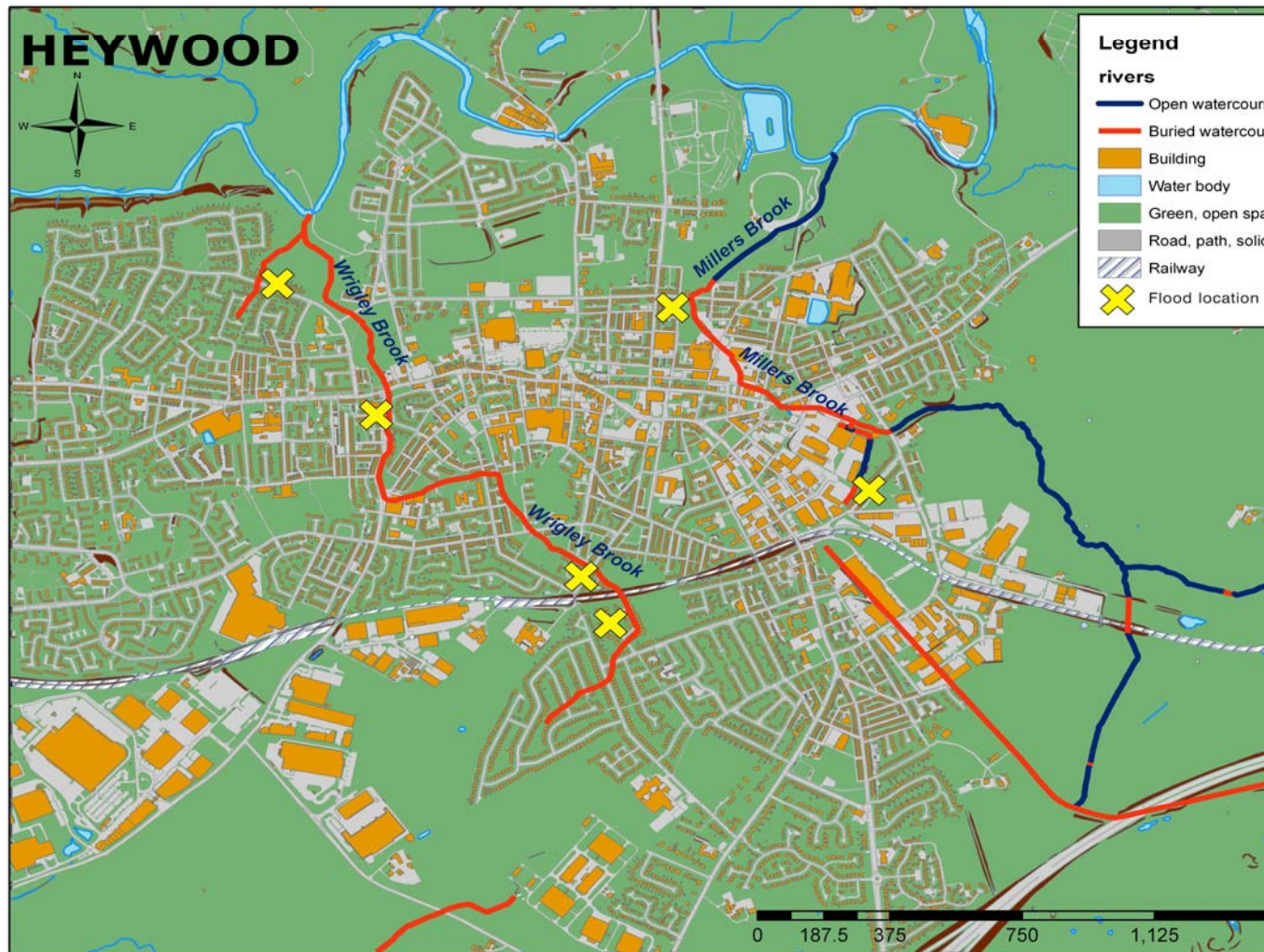
Figure 3 Wrigley Brook and Millers Brook Heywood and location of floods 2004 and 2006
