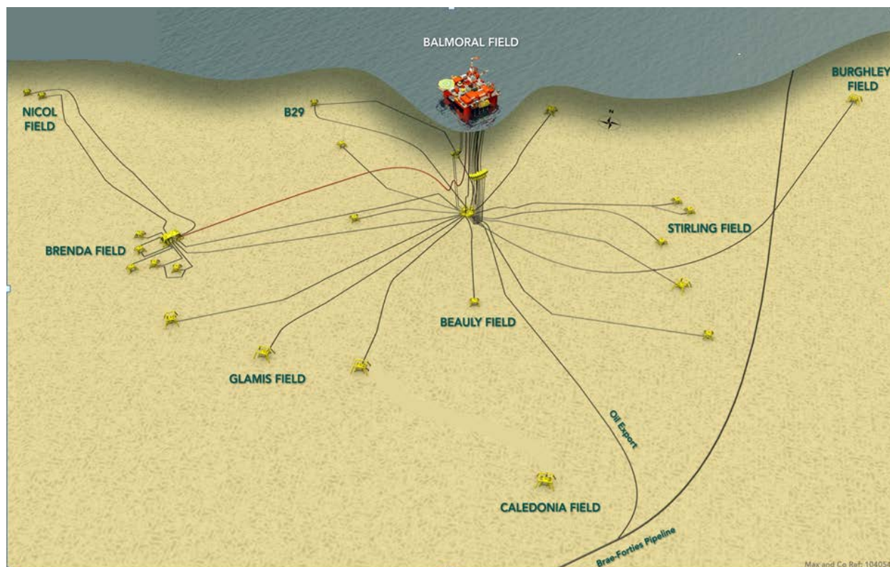
Figure 1.2: Field Layout
