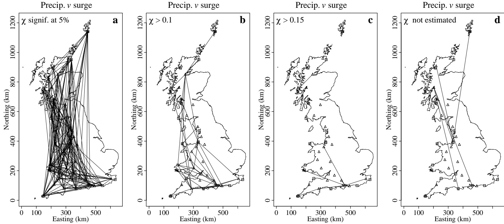
Figure 10 Dependence between precipitation and daily maximum sea surge. Lines connect station-pairs with \chi exceeding a) the 95% point (significant dependence), b) 0.1, and c) 0.15. Figure d) shows lines connecting station-pairs with too few simultaneous observations for \chi to have been estimated.
