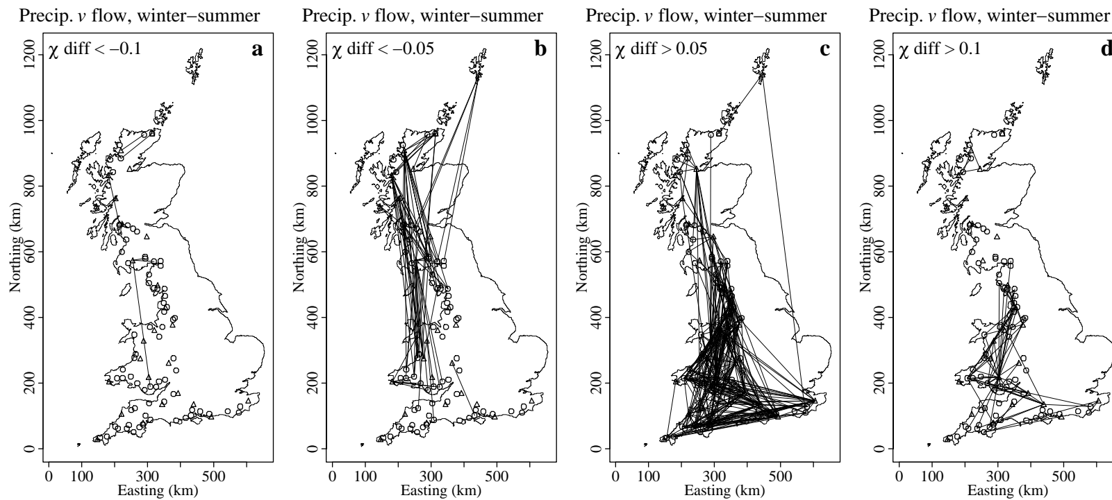
Figure 17 Seasonal difference in dependence ( \chi for winter minus \chi for summer) between precipitation and river flow. Lines connect station-pairs with a difference in \chi a) <-0.1, b) <-0.05, c) >0.05, and d) >0.1.
