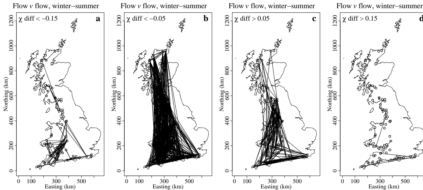
Figure 13 Seasonal difference in inter-station dependence ( \chi for winter minus \chi for summer) in river flow. Lines connect station-pairs with a difference in \chi a) < -0.15 , b) < -0.05 , c) > 0.05 , and d) > 0.15 .
