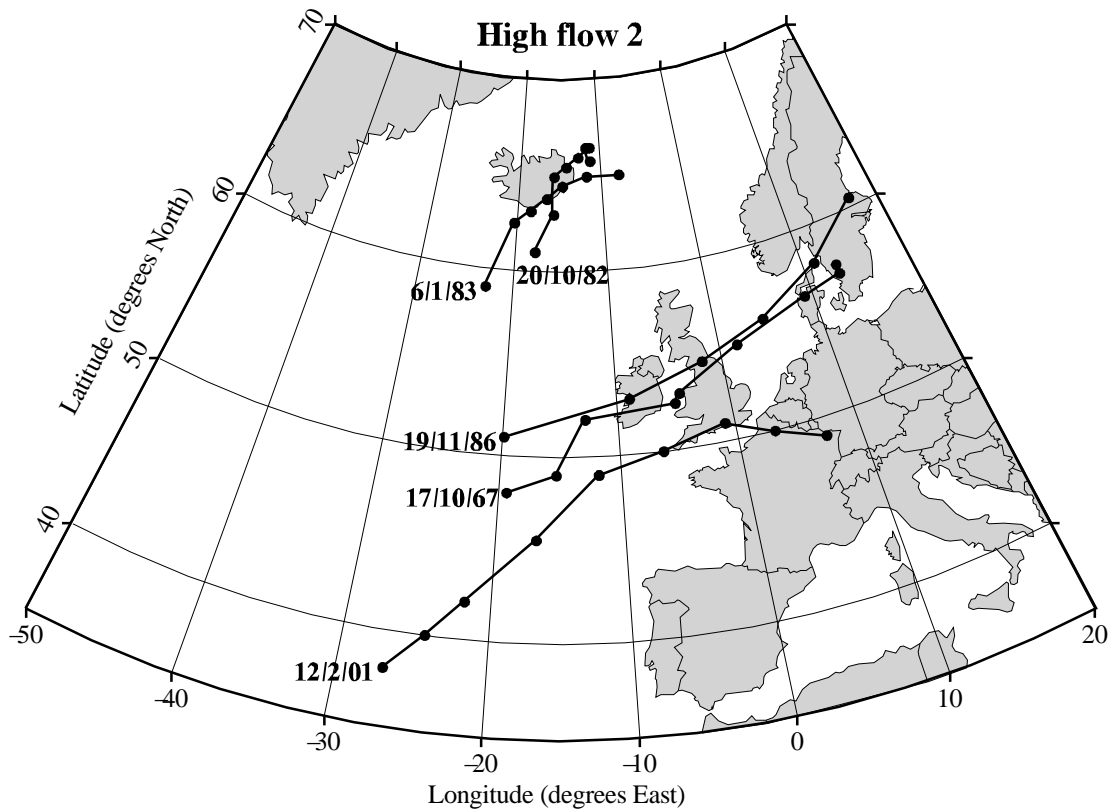
Figure 32 Tracks of five depressions resulting in high river flow and moderate sea surge in southern Wales (Region 2).
