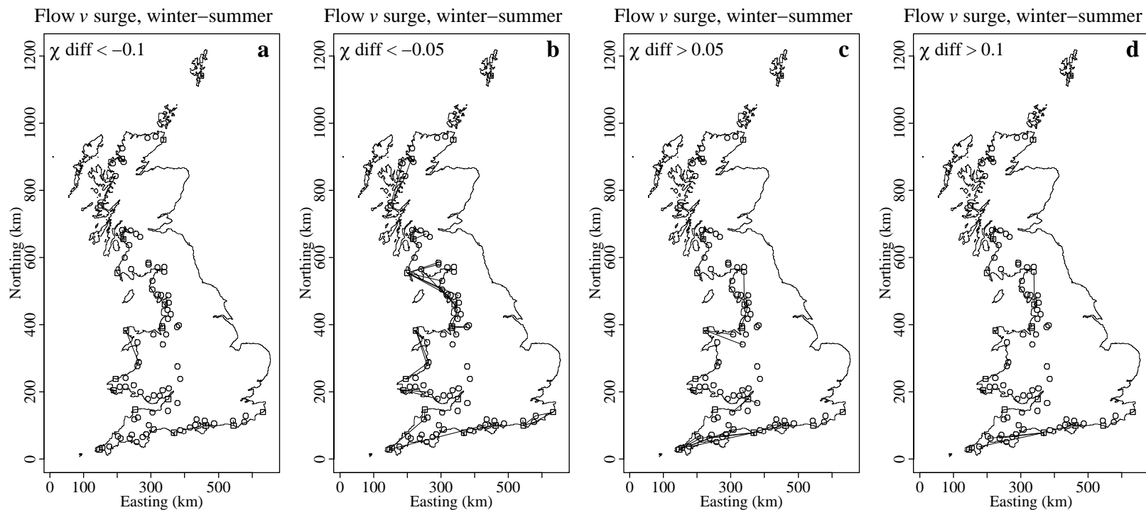
Figure 15 Seasonal difference in dependence ( \chi for winter minus \chi for summer) between river flow and daily maximum sea surge, for neighbouring stations only. Lines connect station-pairs with a difference in \chi a) < -0.1 , b) < -0.05 , c) > 0.05 , and d) > 0.1 .
