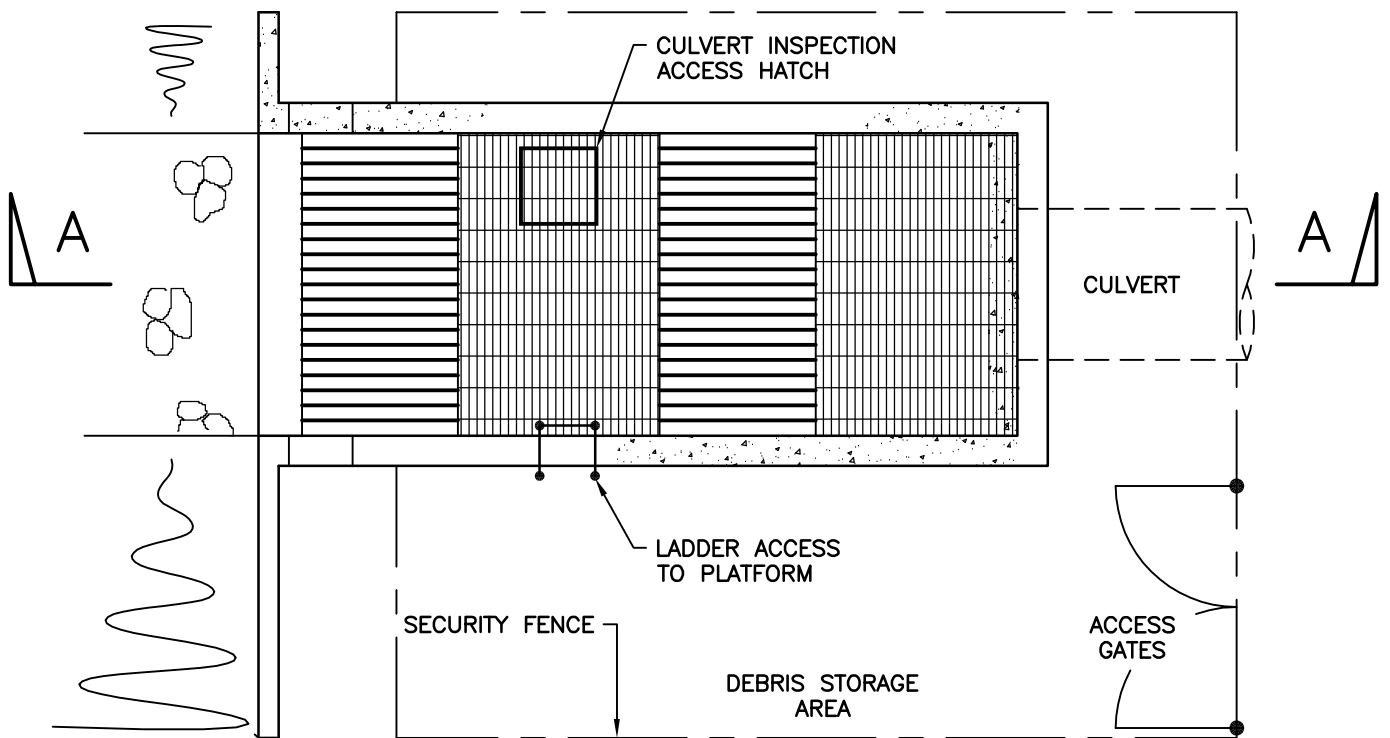
PLAN VIEW
