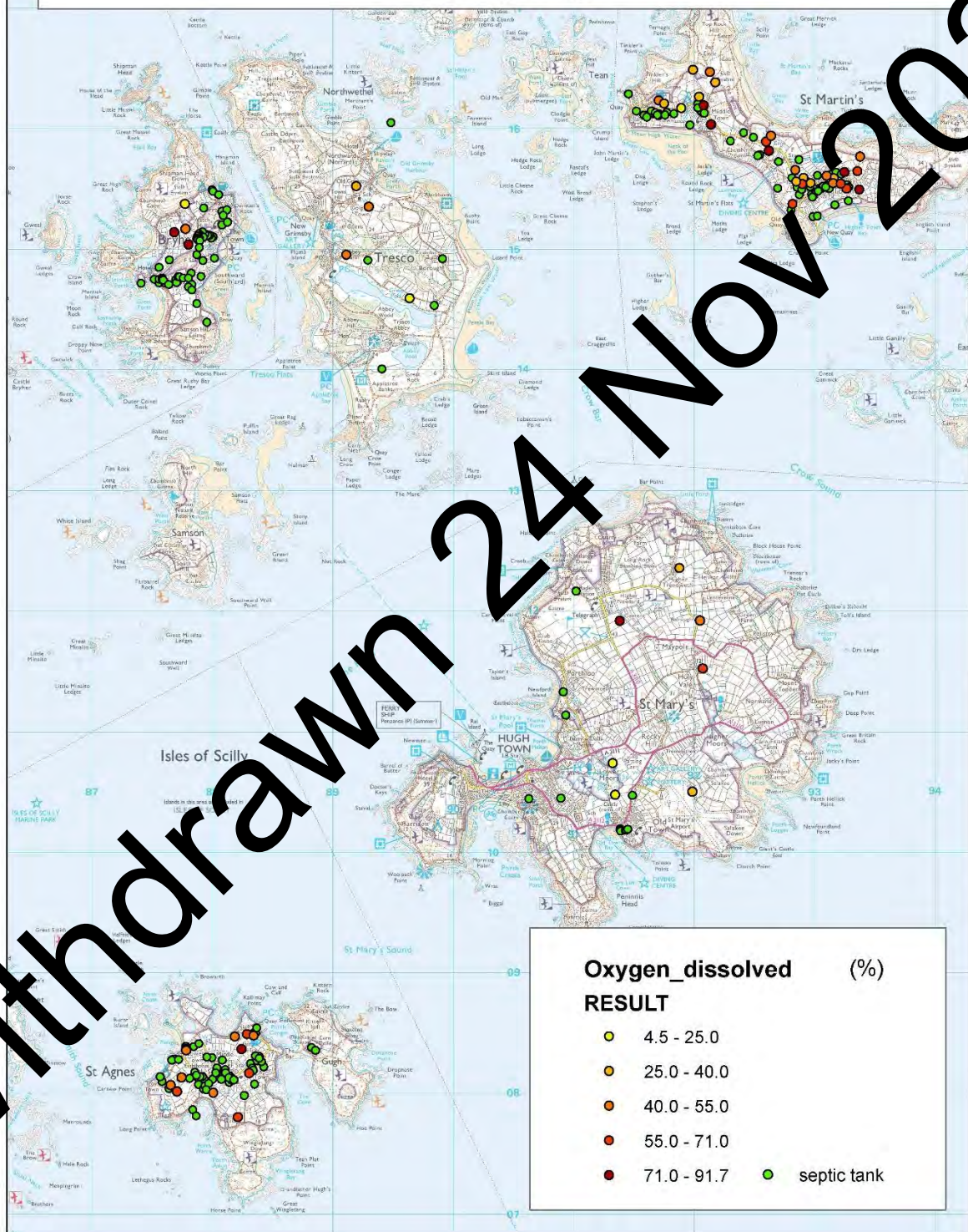
Figure 9: Isles of Scilly dissolved oxygen percentages, November 2015 - January 2016 sampling
