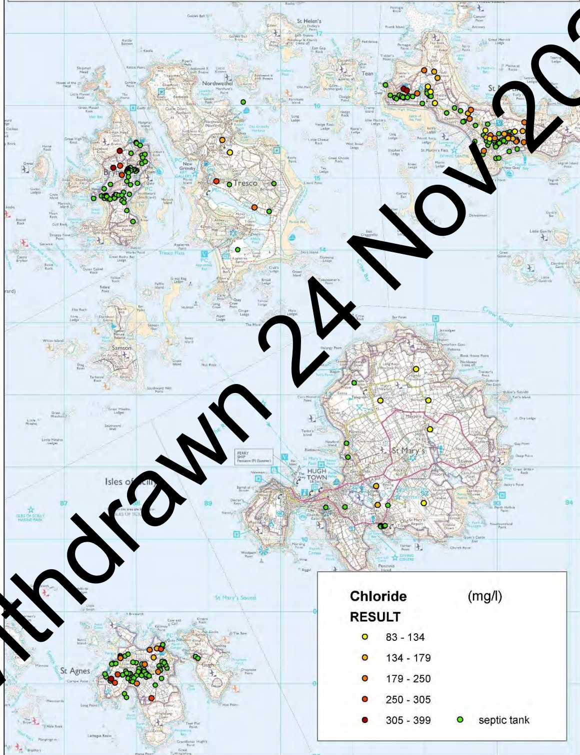
Figure 7: Isles of Scilly chloride concentrations November 2015 - January 2016 sampling
