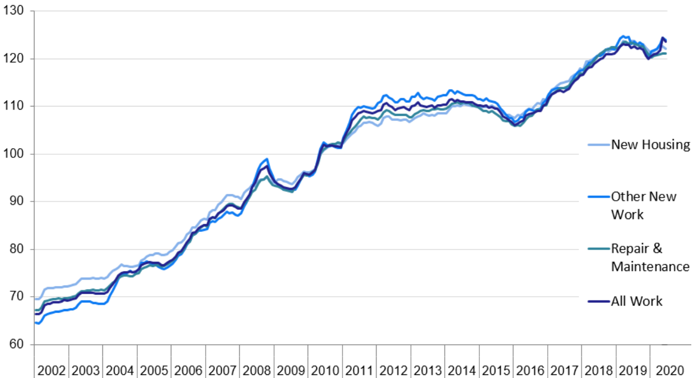
Chart 2: Construction Material Price Indices, UK Index, 2010 = 100
