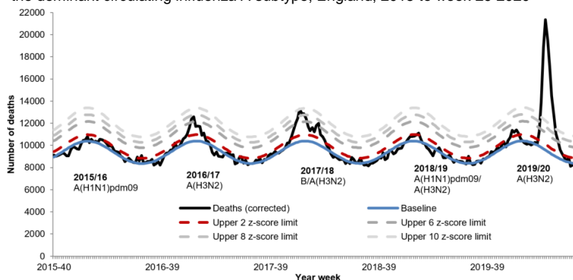
Figure 1: Weekly observed and expected number of all-cause deaths in all ages, with the dominant circulating influenza A subtype, England, 2015 to week 29 2020
