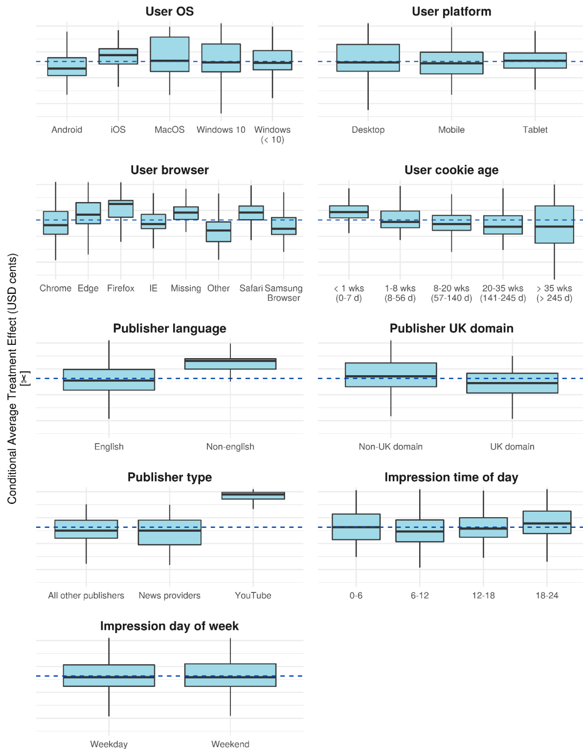
Figure F.4: Heterogeneous effects, causal forests
