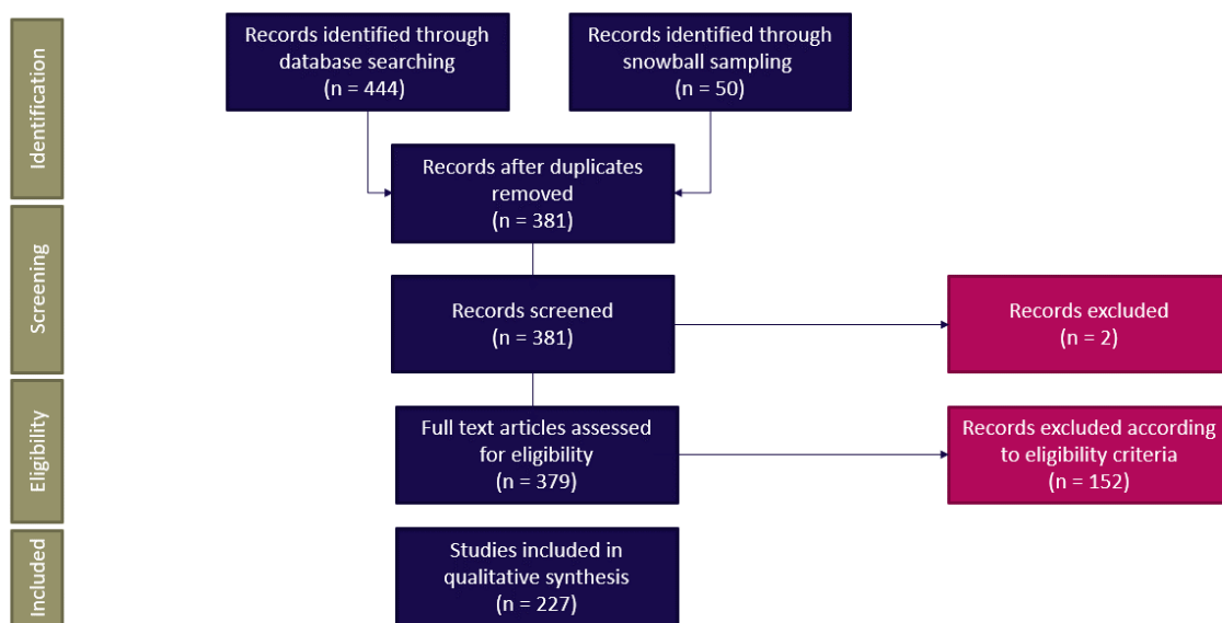
Fig 1. PRISMA diagram
