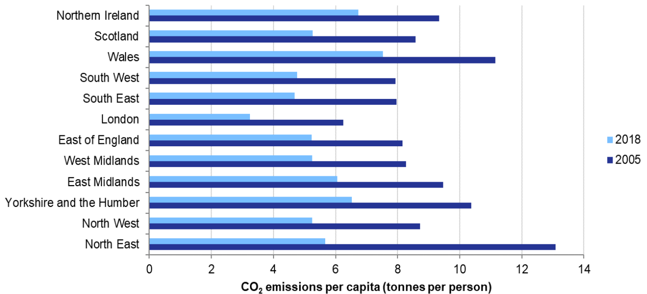
Figure 7: End-user carbon dioxide emissions per capita by region, 2005 and 2018
