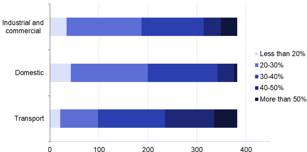
Figure 5: Sectoral breakdown of emissions: Number of UK Local Authorities by proportion of carbon dioxide emissions in each sector (excluding LULUCF), 2018
