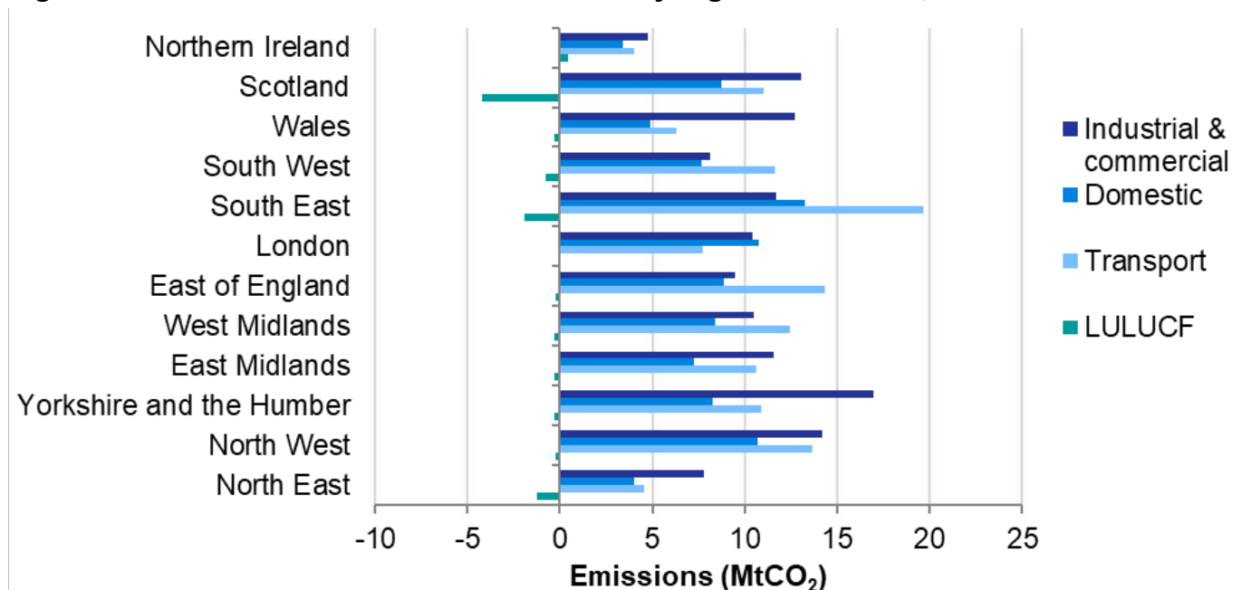
Figure 2: End-user carbon dioxide emissions by region and sector, 2018
