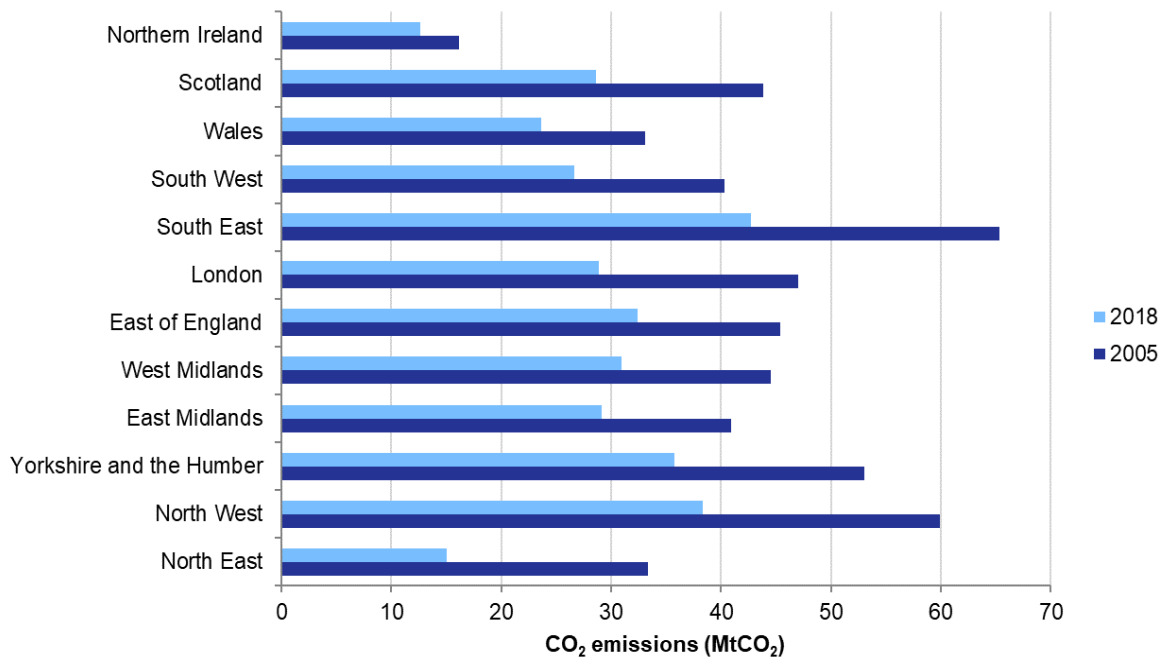
Figure 6: End-user carbon dioxide emissions by region, 2005 and 2018
