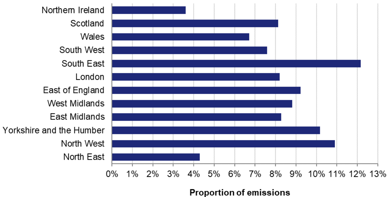
Figure 4: Proportion of UK emissions in each region: 2018
