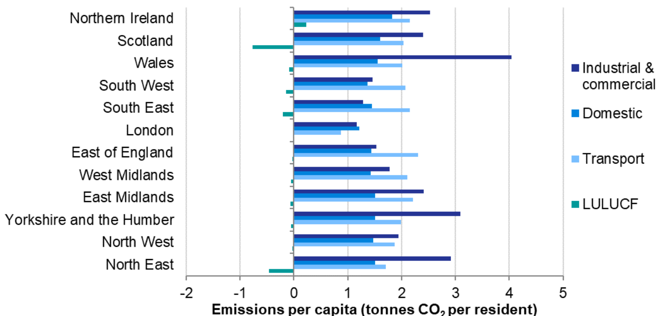
Figure 3: Per capita end-user carbon dioxide emissions by region and sector, 2018
