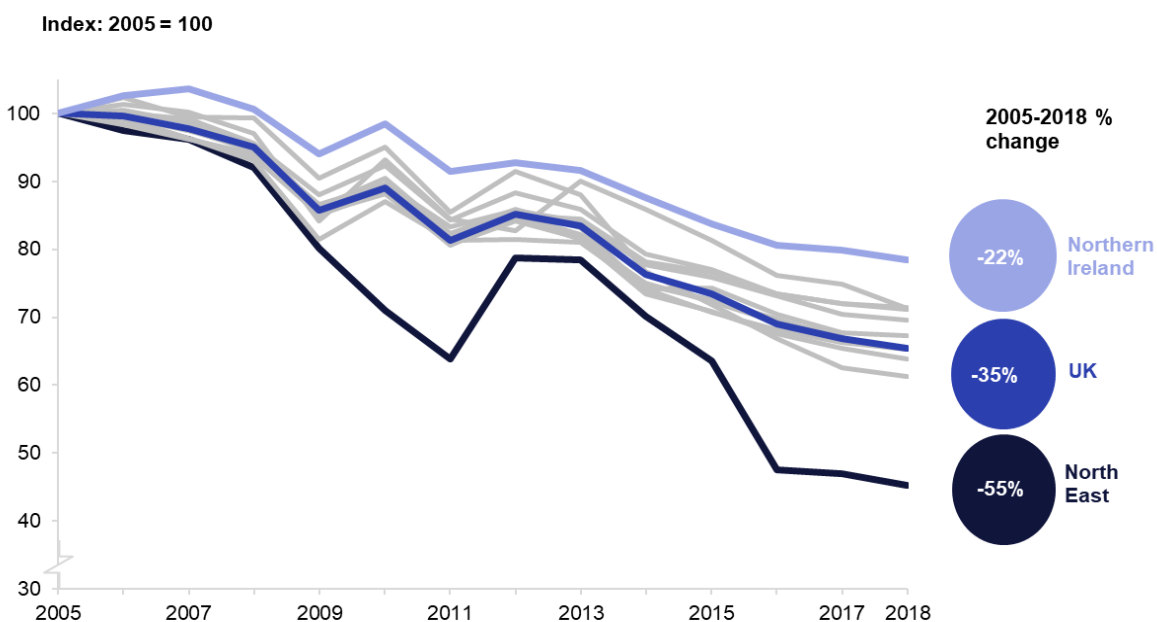
Figure 1: End-user carbon dioxide emissions by region
