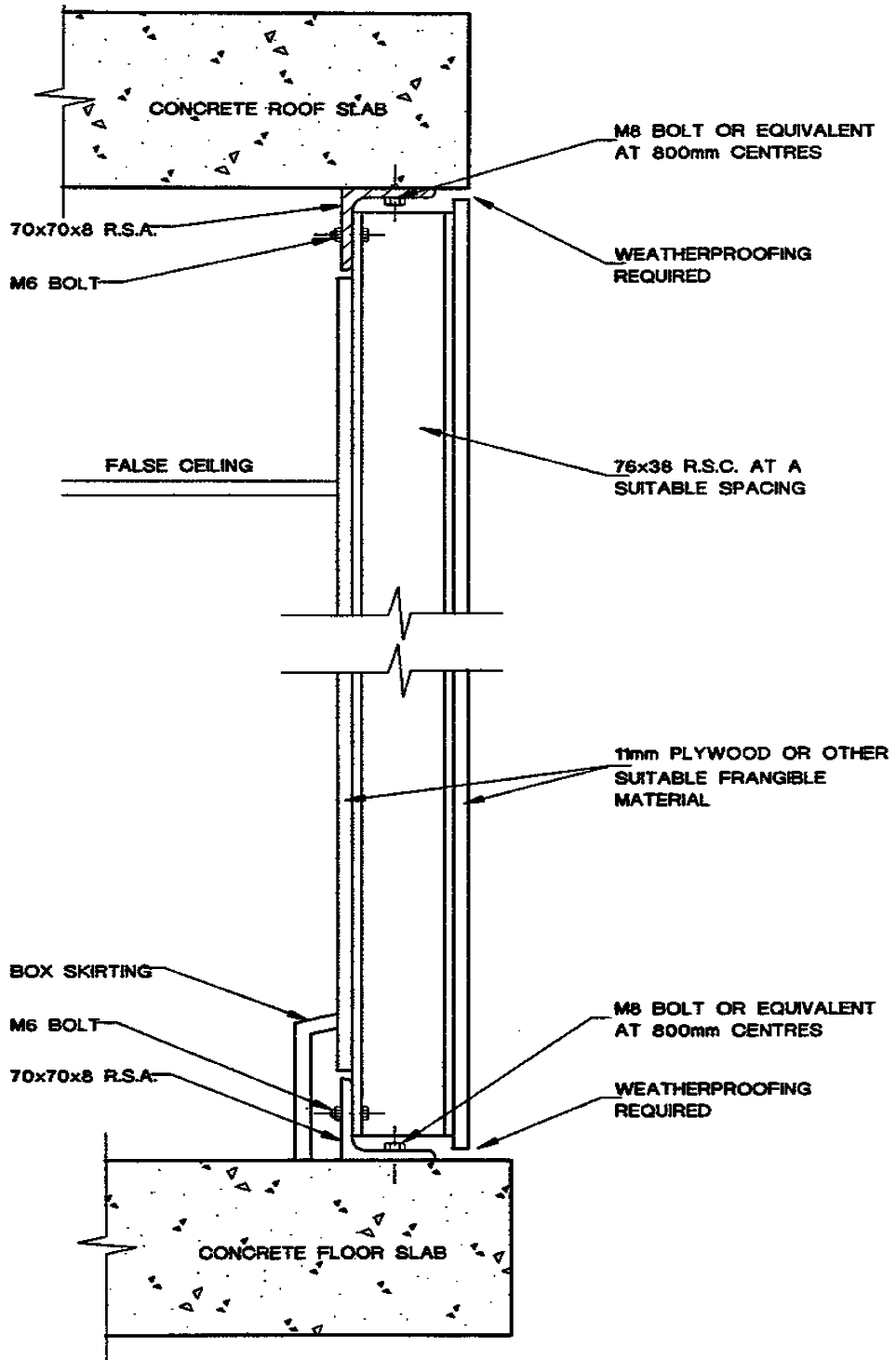
Fig 2 Alternative Blow-out Panel
