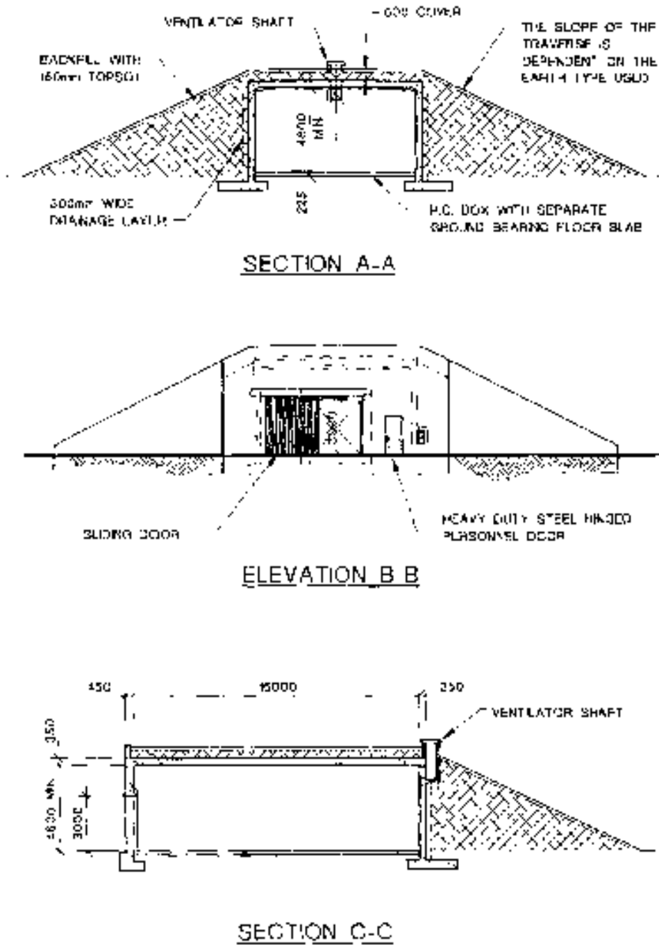
Fig 2 Standard Storehouse - UK Box Igloo (Single Bay)
