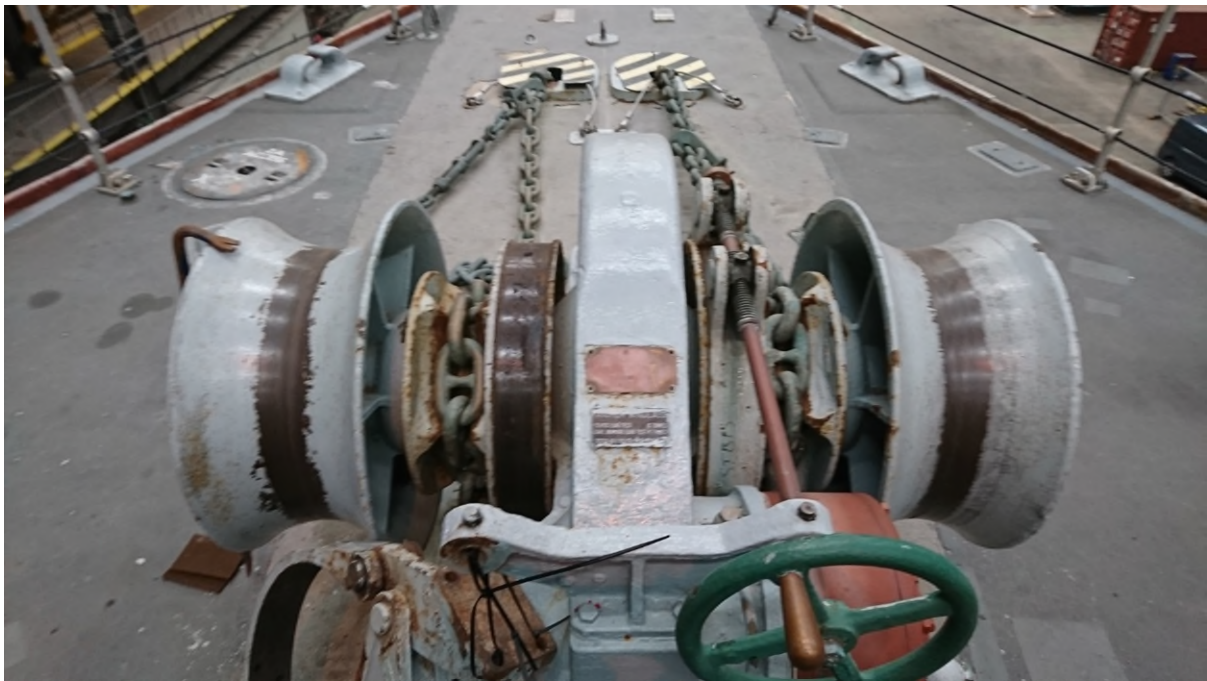
Focs'le anchor windlass and cable holder port. Note, only one set of cable and anchor will remain.
