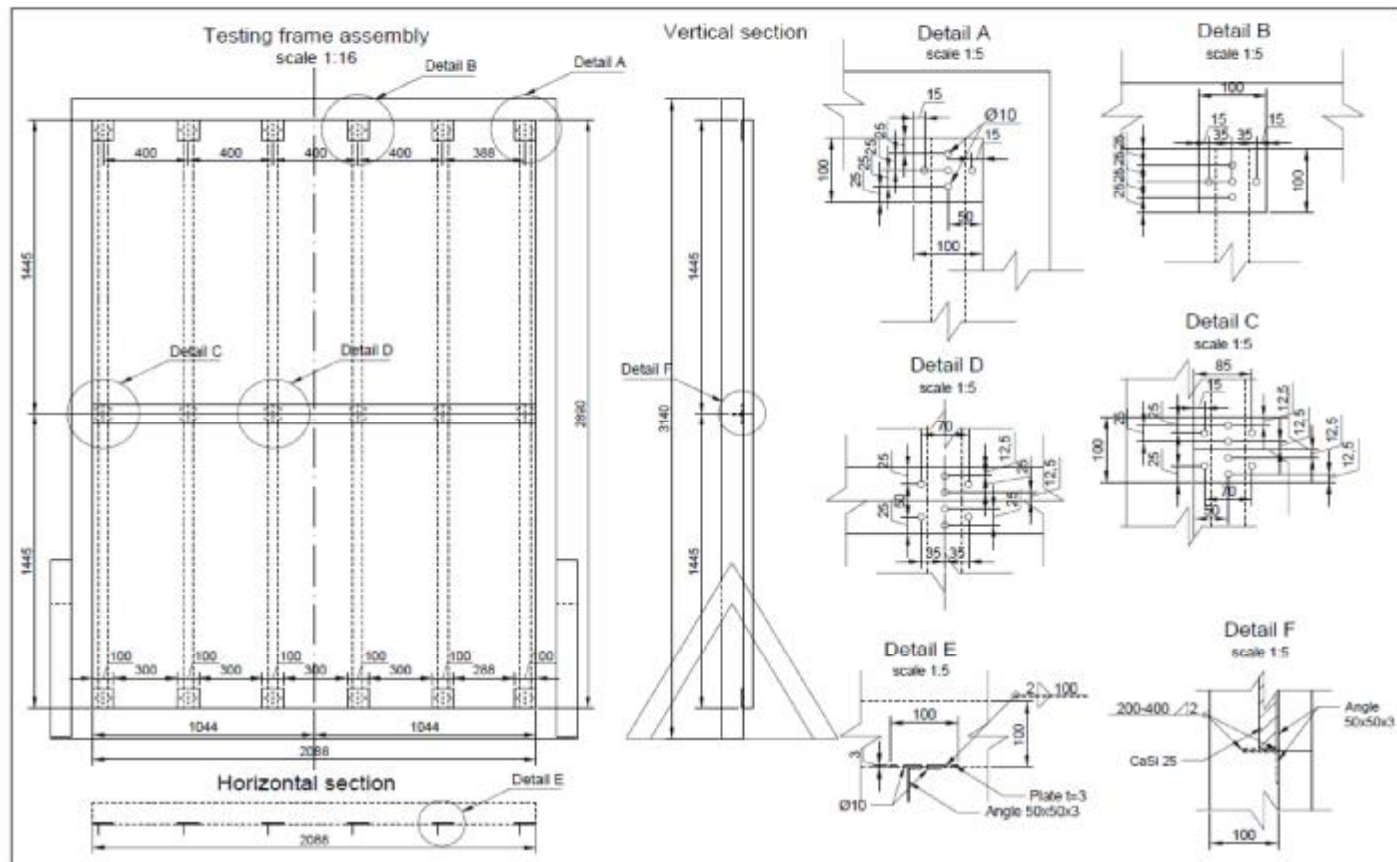
Figure C1 – Proposed experimental frame assembly
