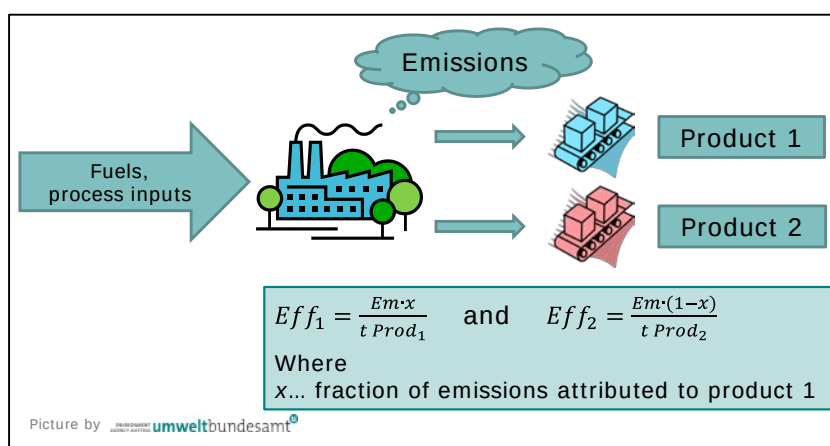
Figure 7: For benchmarking of an installation with two products, an approach is required to split emissions according to the two products. (Eff...efficiency; Em...emissions)
