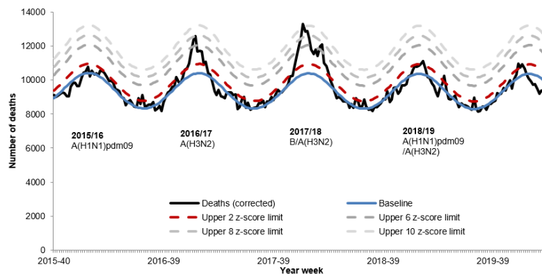
Figure 1: Weekly observed and expected number of all-cause deaths in all ages, with the dominant circulating influenza A subtype, England, 2015 to week 11 2020
