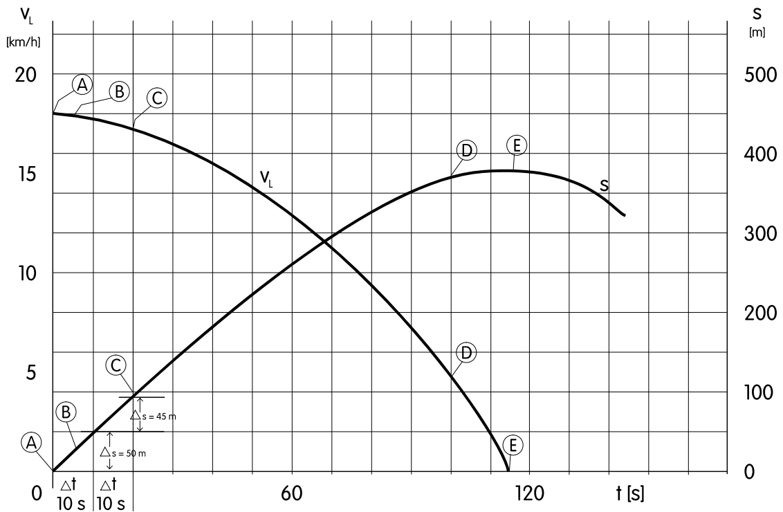
Figure 1: Stopping manoeuvre
