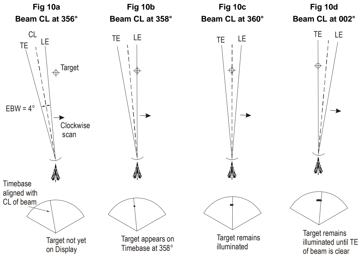
11-8 Fig 10 Effective Beamwidth
