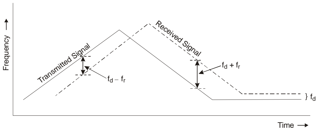
11-12 Fig 12 Principle of FM Ranging
