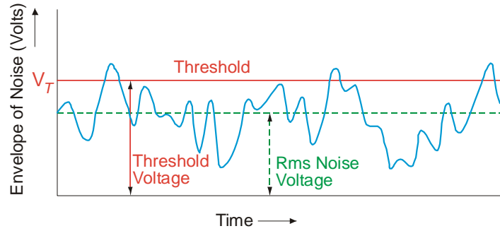
11-3 Fig 3 False Alarms Due to Noise
