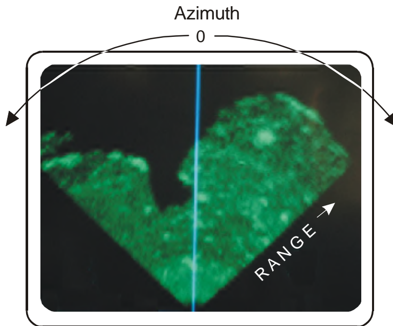
11-1 Fig 4 Sector PPI Display
