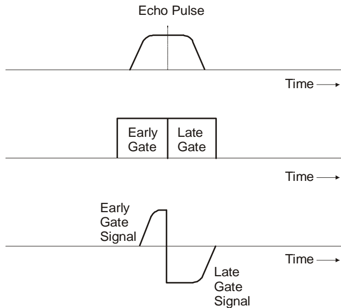
11-6 Fig 4 Range Tracking by Split Range Gate
