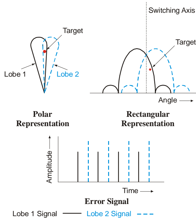
11-6 Fig 3 Sequential Lobing
