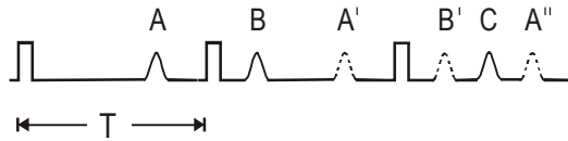
Fig 3a Multiple-time-around Echoes
