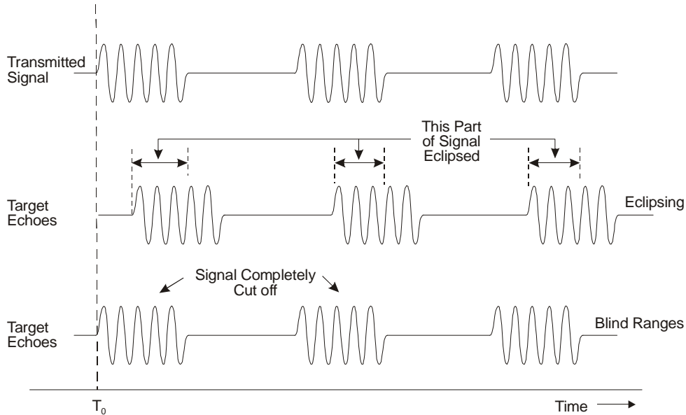
11-12 Fig 4 Eclipsing and Blind Ranges
