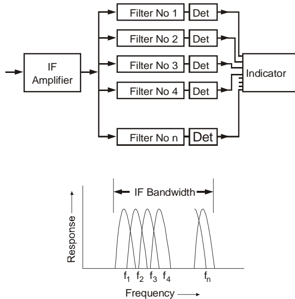
11-4 Fig 4 IF/Filter Bandwidths
