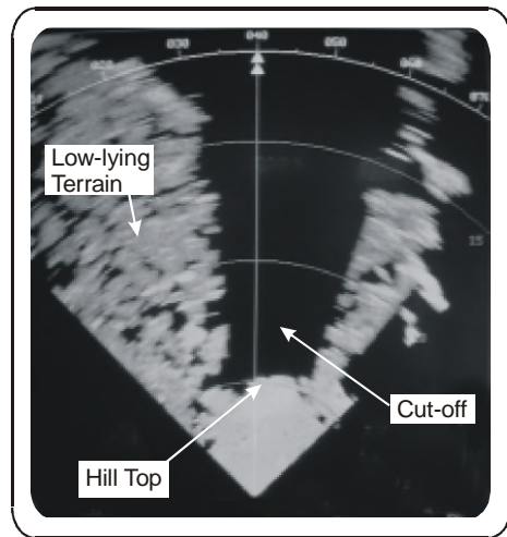
Fig 29b Radar Display
