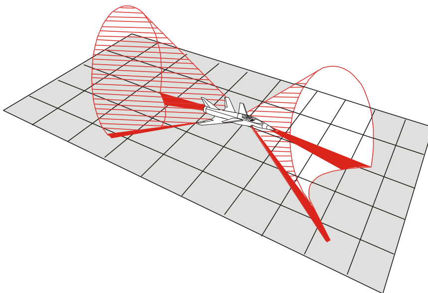
11-7 Fig 9 A Practical Doppler Beam Shape
