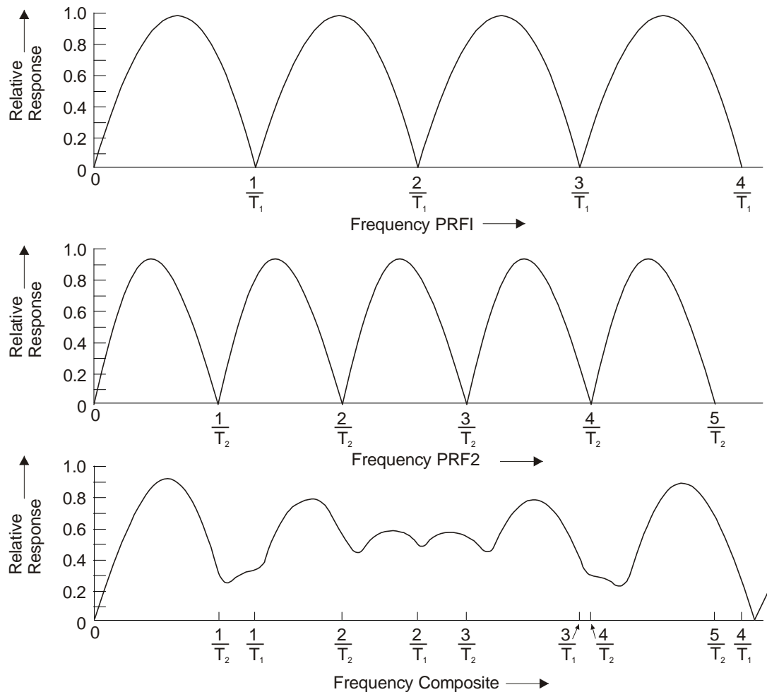
11-5 Fig 1 Frequency Response for Time-shared PRFs
