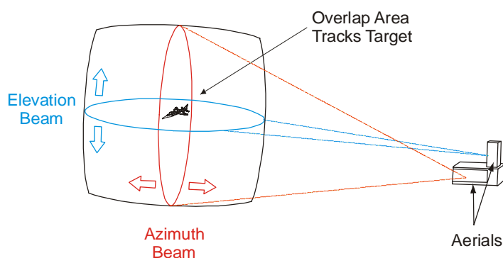
11-6 Fig 5 Electro-mechanical Track-while-scan Radar
