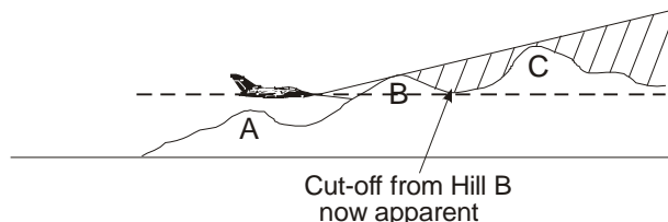
Fig 30b Development of Cut-off as Range Decreases
