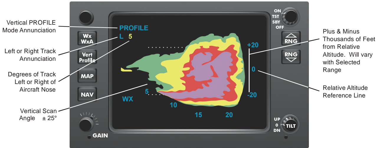
11-11 Fig 5 'Profile' Scan
