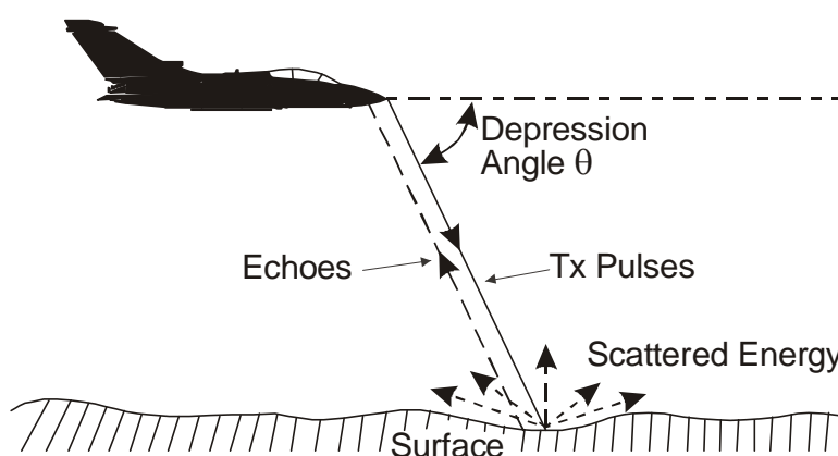
11-7 Fig 3 Principle of Doppler Groundspeed Measurement
