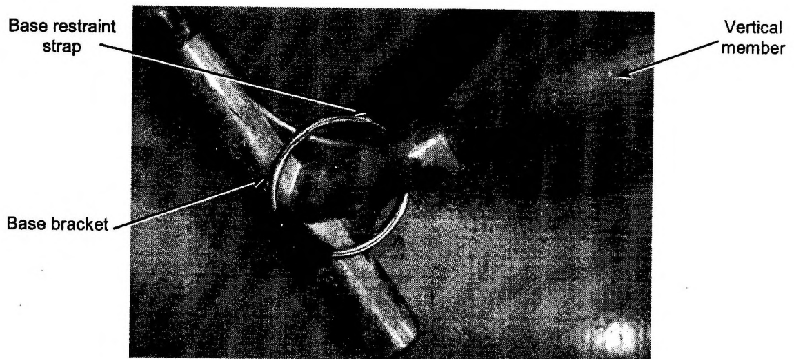
Fig 16 Base restraint strap fixing
