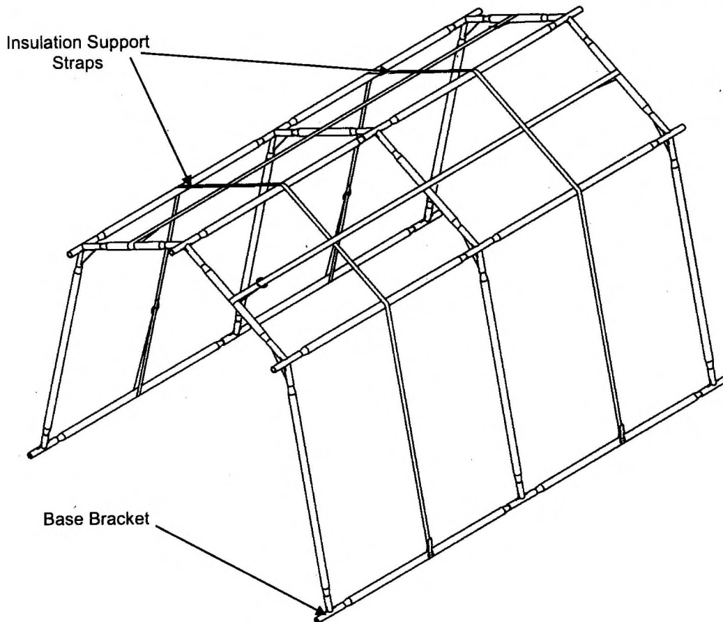
Fig 15 Frame with insulation support strap
