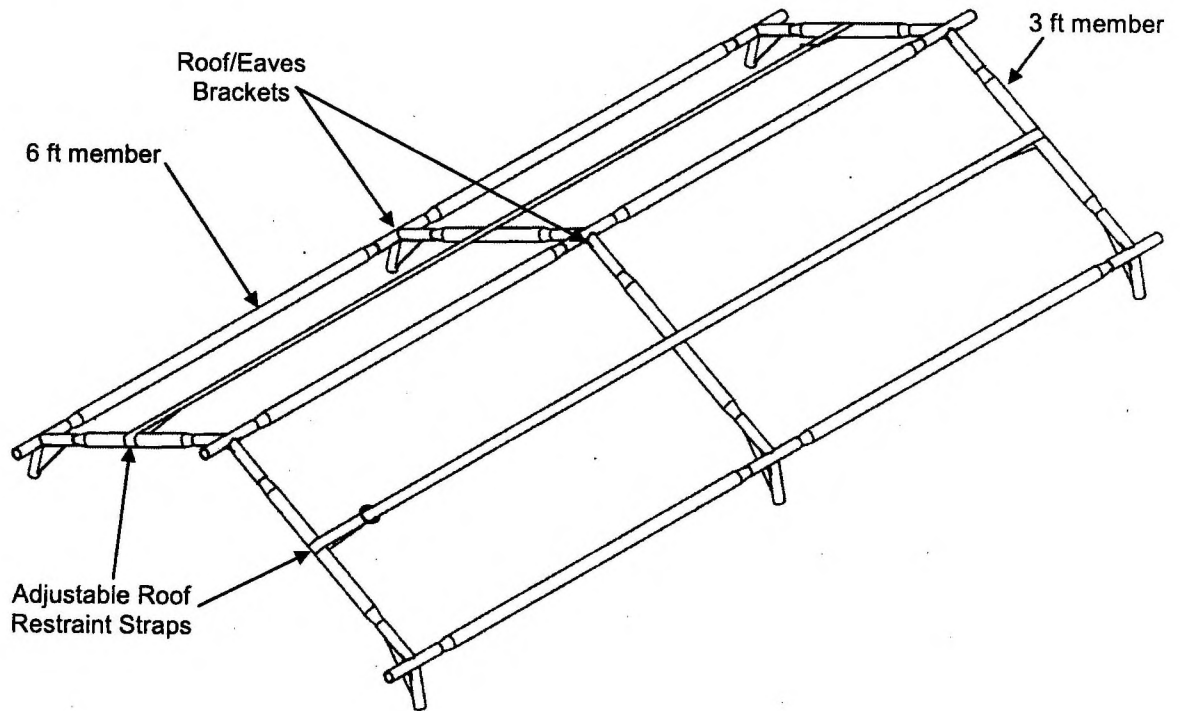
Fig 10 Roof frame assembly
