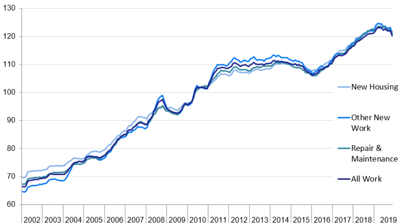
Chart 1: Construction Material Price Indices, UK
