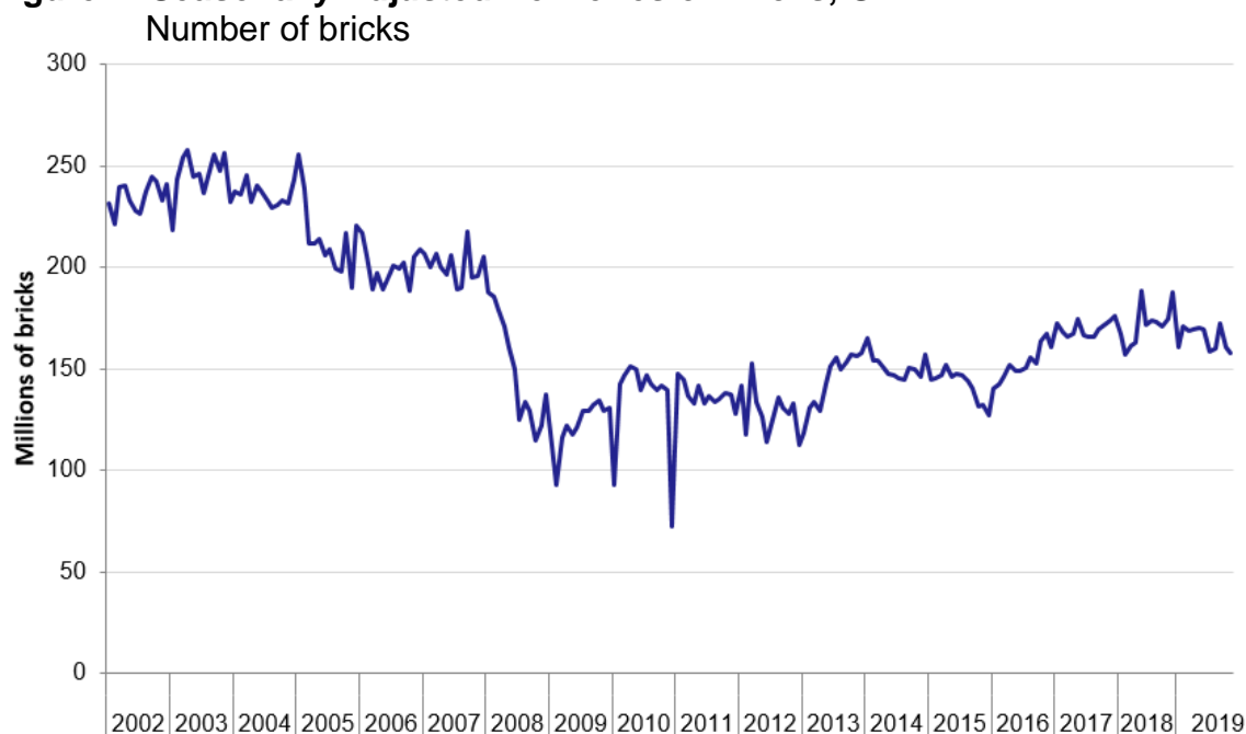
Figure 1: Seasonally Adjusted Deliveries of Bricks, GB
