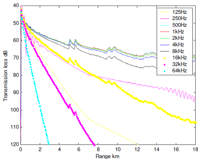
Figure 7: Predicted propagation loss to the south-west of the proposed survey area in typical summer conditions
