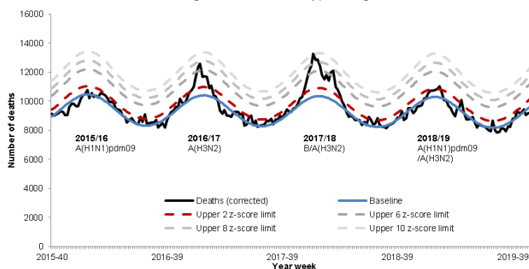
Figure 1: Weekly observed and expected number of all-cause deaths in all ages, with the dominant circulating influenza A subtype, England, 2015 to week 47 2019
