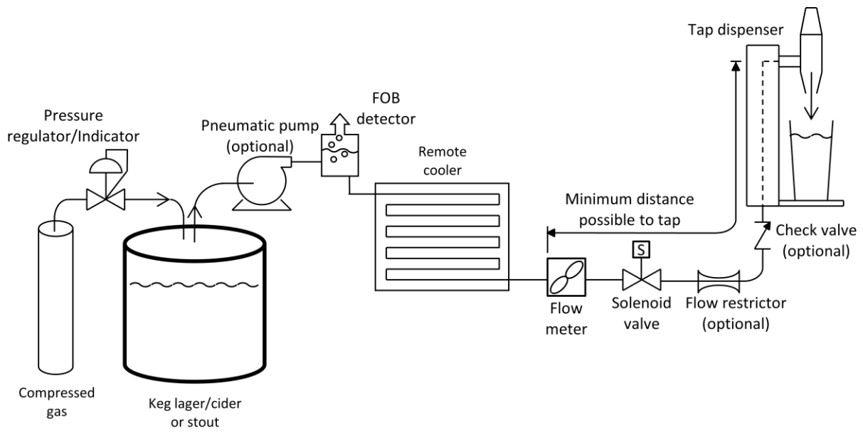
Figure 3 - Product flow schematic
