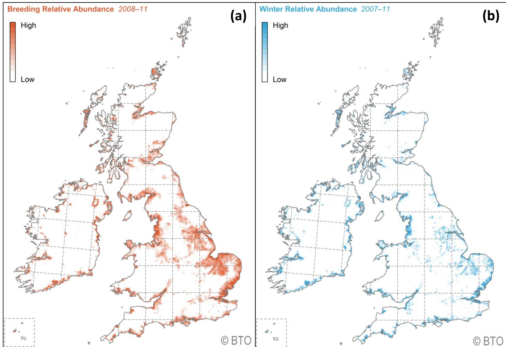
Figure 2 Relative abundance of the British and Irish Shelduck population during a) the breeding season; and b) the non-breeding season. Distribution maps from Bird Atlas 2007-11 which is a joint project between BTO, BirdWatch Ireland and the Scottish Ornithologists' Club. Maps reproduced with permission from the BTO.
