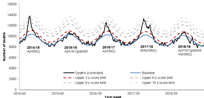
Figure 1: Weekly observed and expected number of all-cause deaths in all ages, with the dominant circulating influenza A subtype, England, 2014 to week 32 2019
