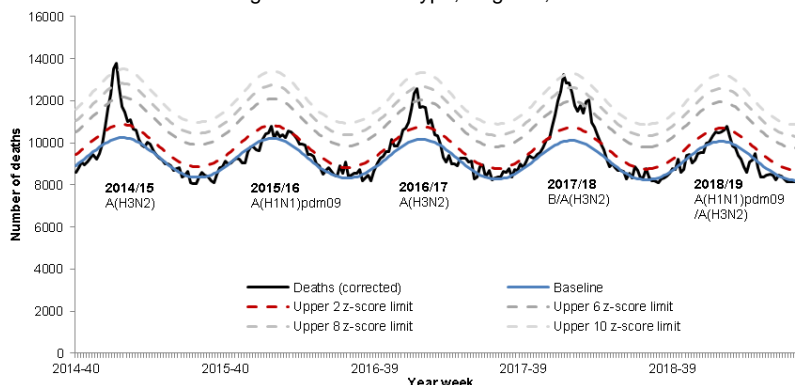
Figure 1: Weekly observed and expected number of all-cause deaths in all ages, with the dominant circulating influenza A subtype, England, 2014 to week 30 2019
