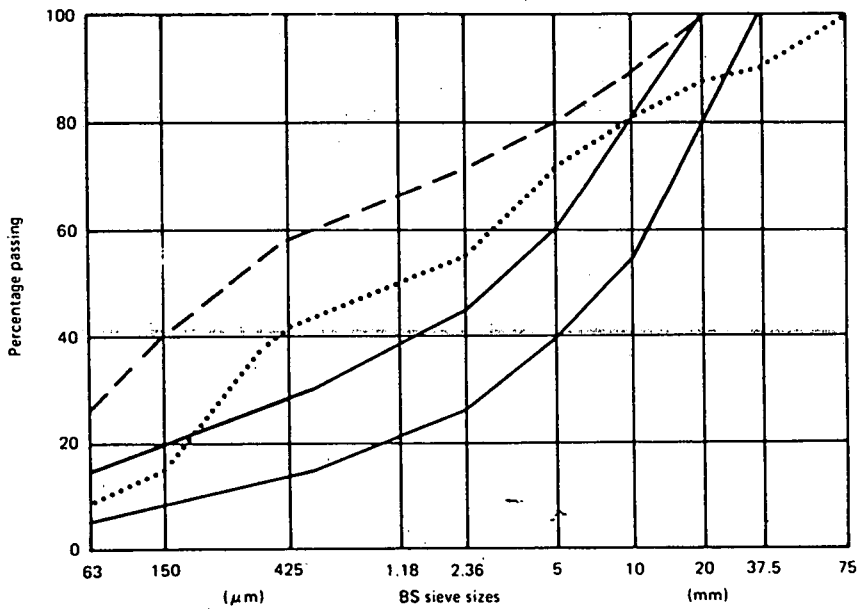
FIGURE 3 Particle size distribution of powder calcrete BG6 before and after field compaction.
