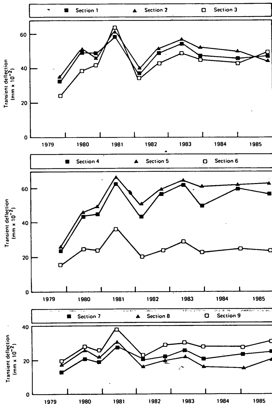
FIGURE 12 Mean transient deflection values versus time.
