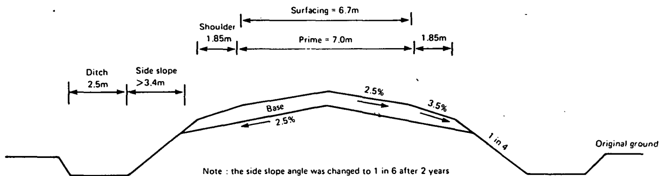
FIGURE 7 Typical cross-section and pavement details.
