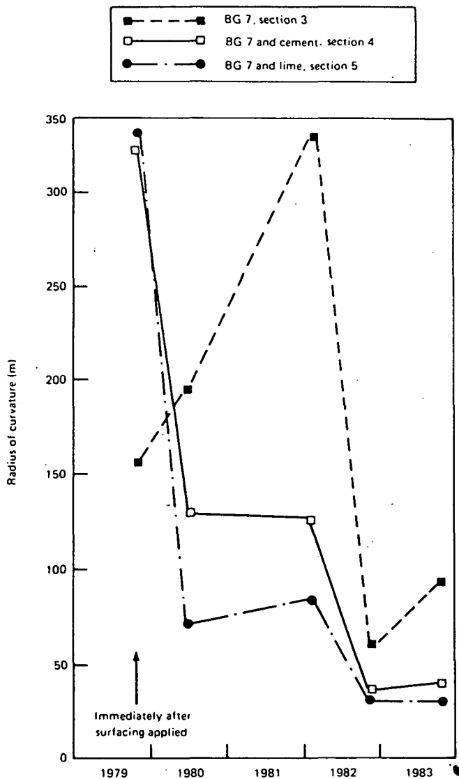
FIGURE 14 Radius of curvature history for Sections 3, 4, and 5.
