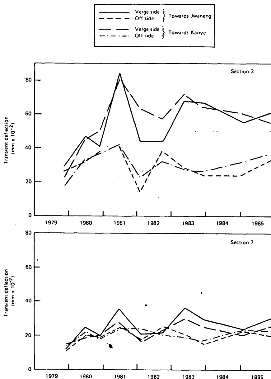
FIGURE 13 Deflection history for Sections 3 and 7.
