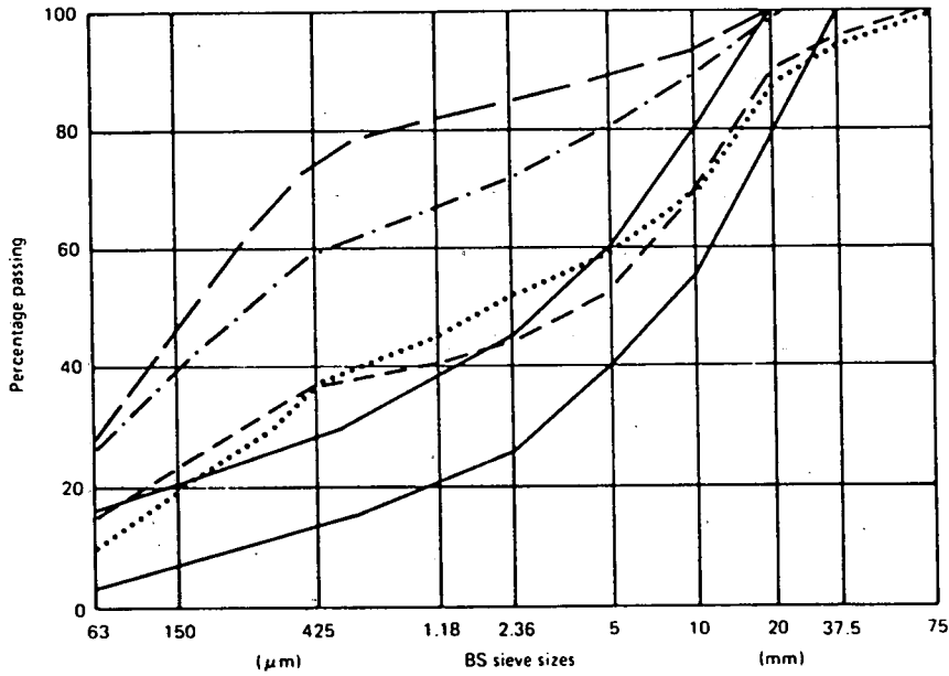
FIGURE 2 Mean particle size distribution of samples of four untreated calcretes taken after field compaction.
