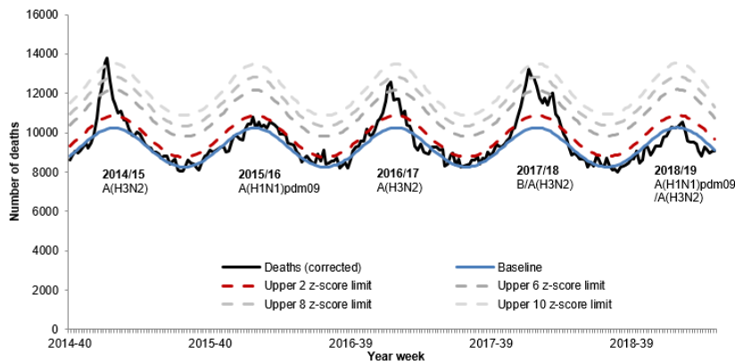
Figure 1: Weekly observed and expected number of all-cause deaths in all ages, with the dominant circulating influenza A subtype, England, 2014 to week 18 2019
