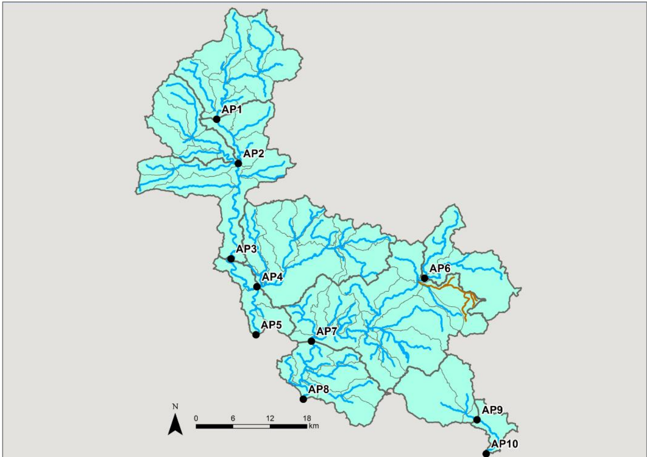
Map 6: Water resource reliability of the Cherwell, Thame and Wye ALS expressed as percentage of time available
