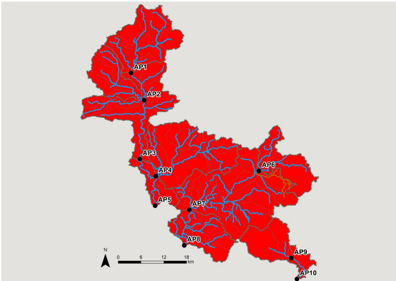
Map 10: Water resource availability colours at Q70 for the Cherwell, Thame and Wye ALS with Thames bespoke licensing strategy applied.
