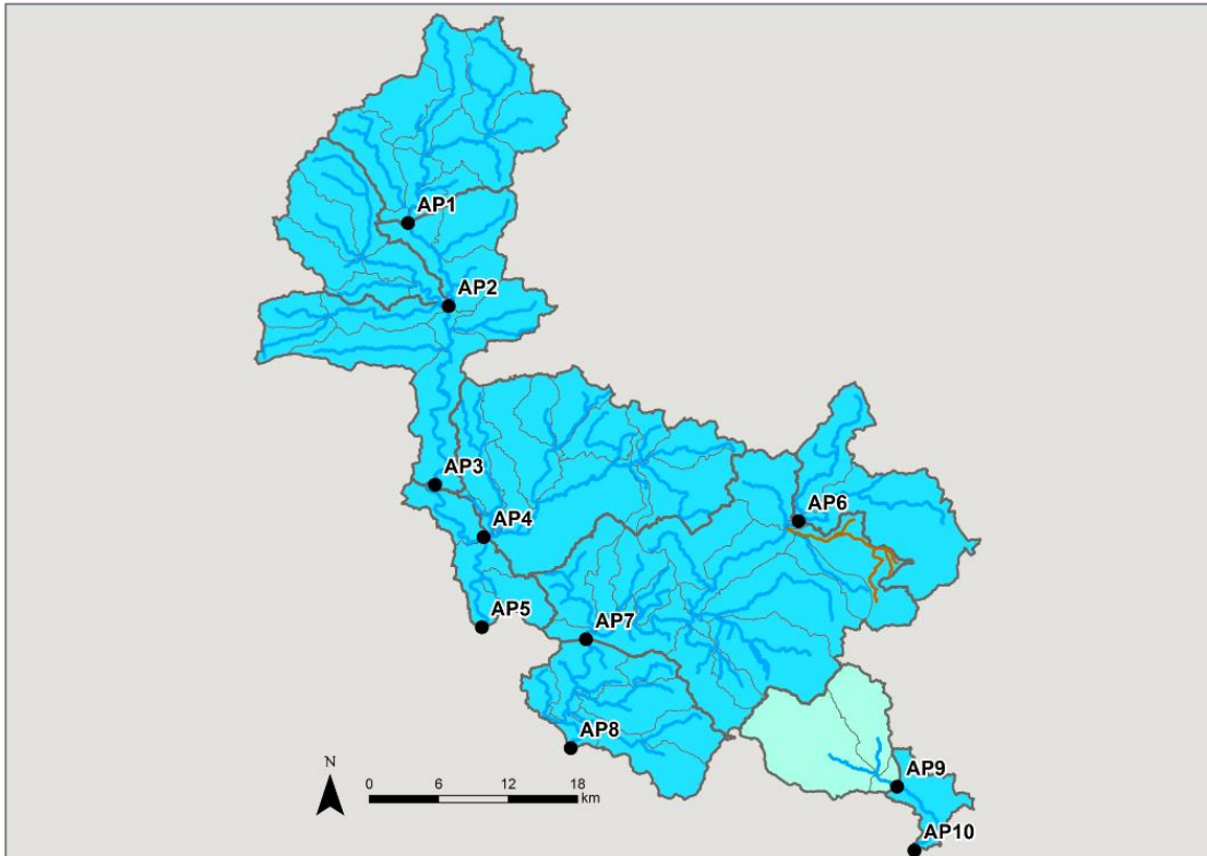
Map 12: Water resource reliability of the Cherwell, Thame and Wye ALS expressed as percentage of time available with the Thames bespoke licensing strategy applied.
