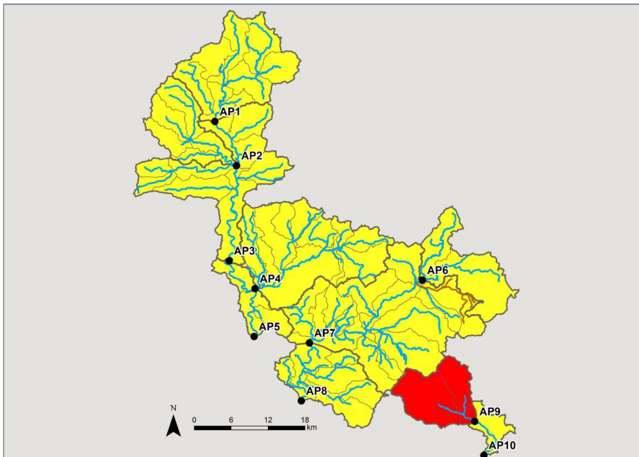
Map 2: Water resource availability colours at Q30 for the Cherwell, Thame and Wye ALS.
