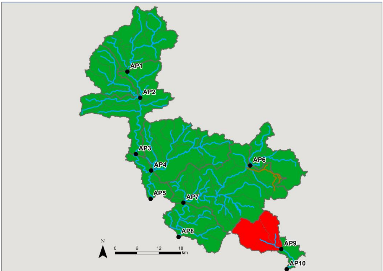
Map 8: Water resource availability colours at Q30 for the Cherwell, Thame and Wye ALS with the Thames bespoke licensing strategy applied.
