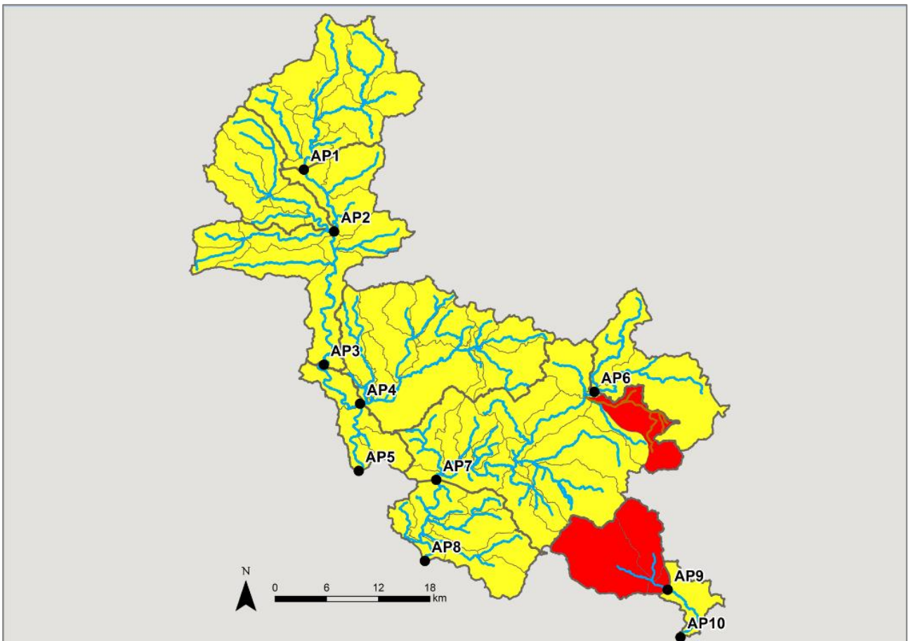
Map 9: Water resource availability colours at Q50 for the Cherwell, Thame and Wye ALS with the Thames bespoke licensing strategy applied.
