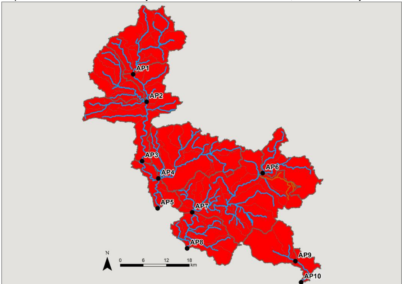
Map 4: Water resource availability colours at Q70 for the Cherwell, Thame and Wye ALS.
