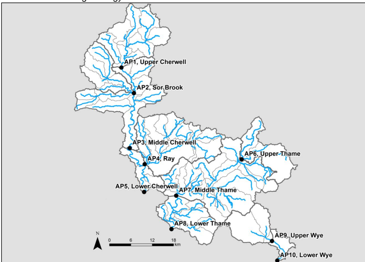
Map 1: The Cherwell, Thame and Wye ALS area showing the Assessment Points (APs) used in this licensing strategy.
