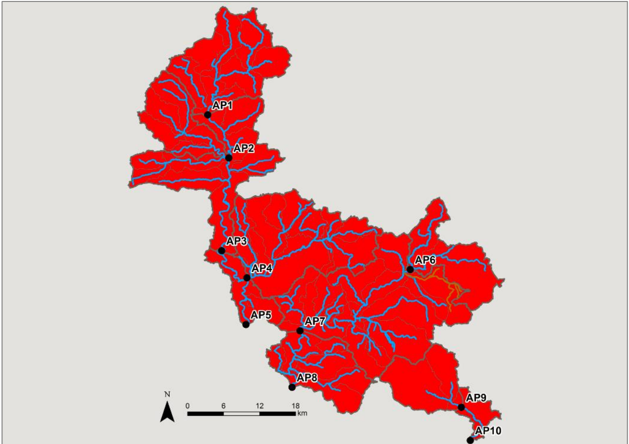
Map 3: Water resource availability colours at Q50 for the Cherwell, Thame and Wye ALS.
