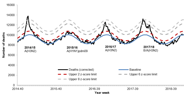
Figure 1: Weekly observed and expected number of all-cause deaths in all ages, with the dominant circulating influenza A subtype, England, 2014 to week 05 2019
