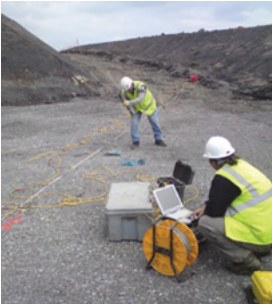
Seismic refraction and reflection. Image courtesy of AGS.
