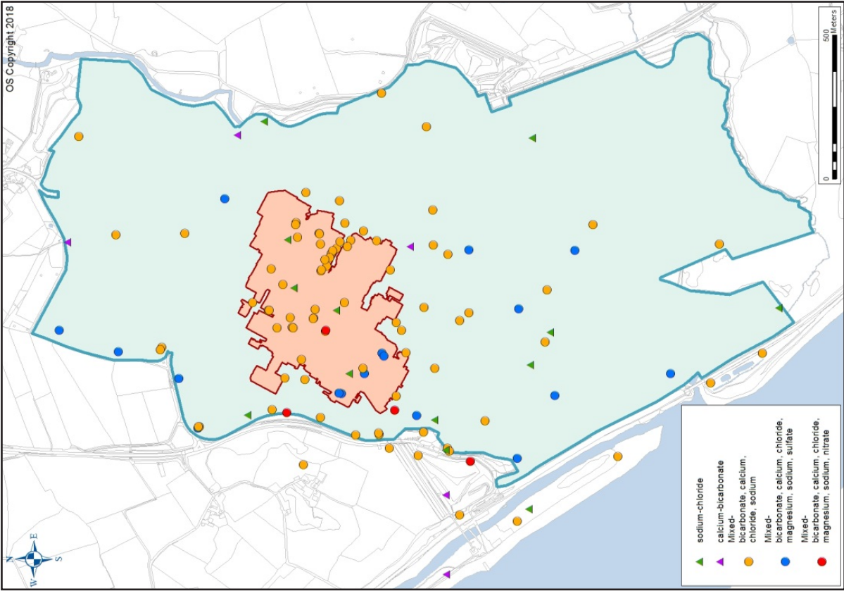
Figure 9. Groundwater types identified from samples collected between April 2017 and June 2017 (where multi-depth installations are included the deeper piezometer-P1- is shown)
