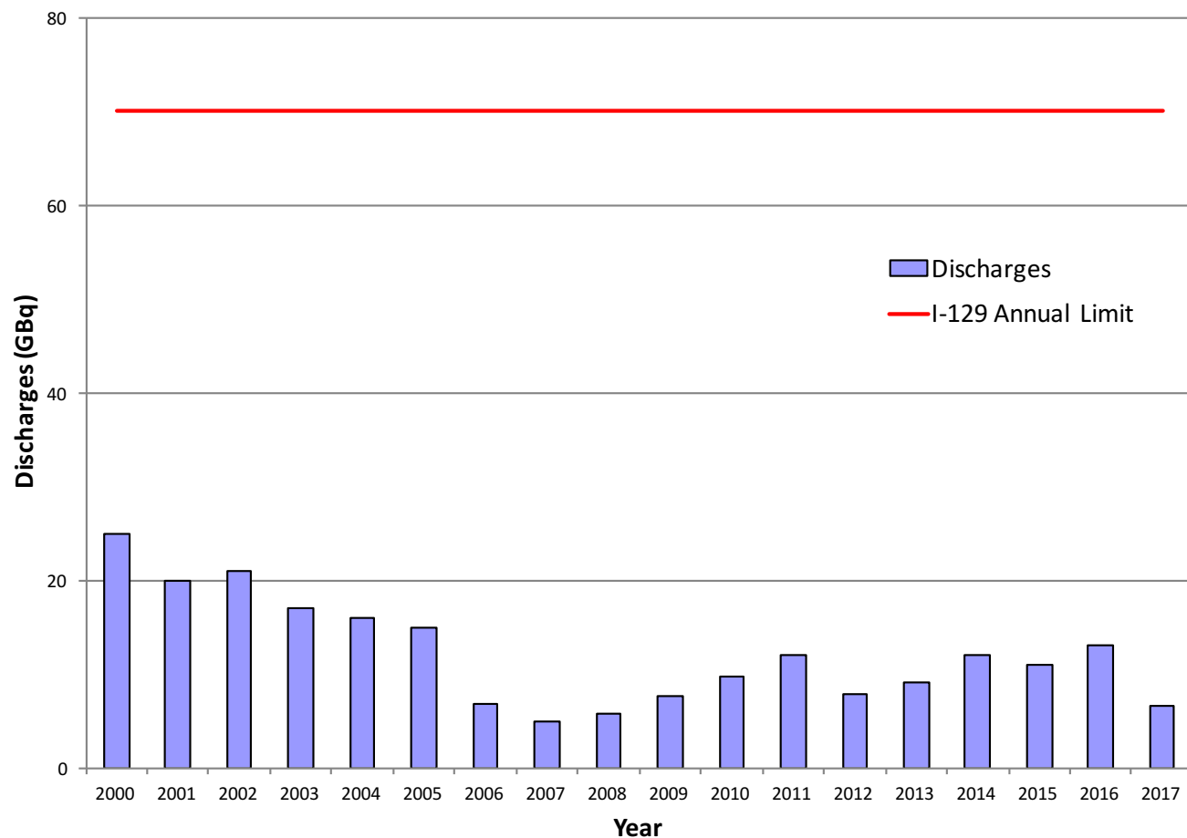
Figure 3b. Annual aerial discharges of Iodine-129 (GBq)
